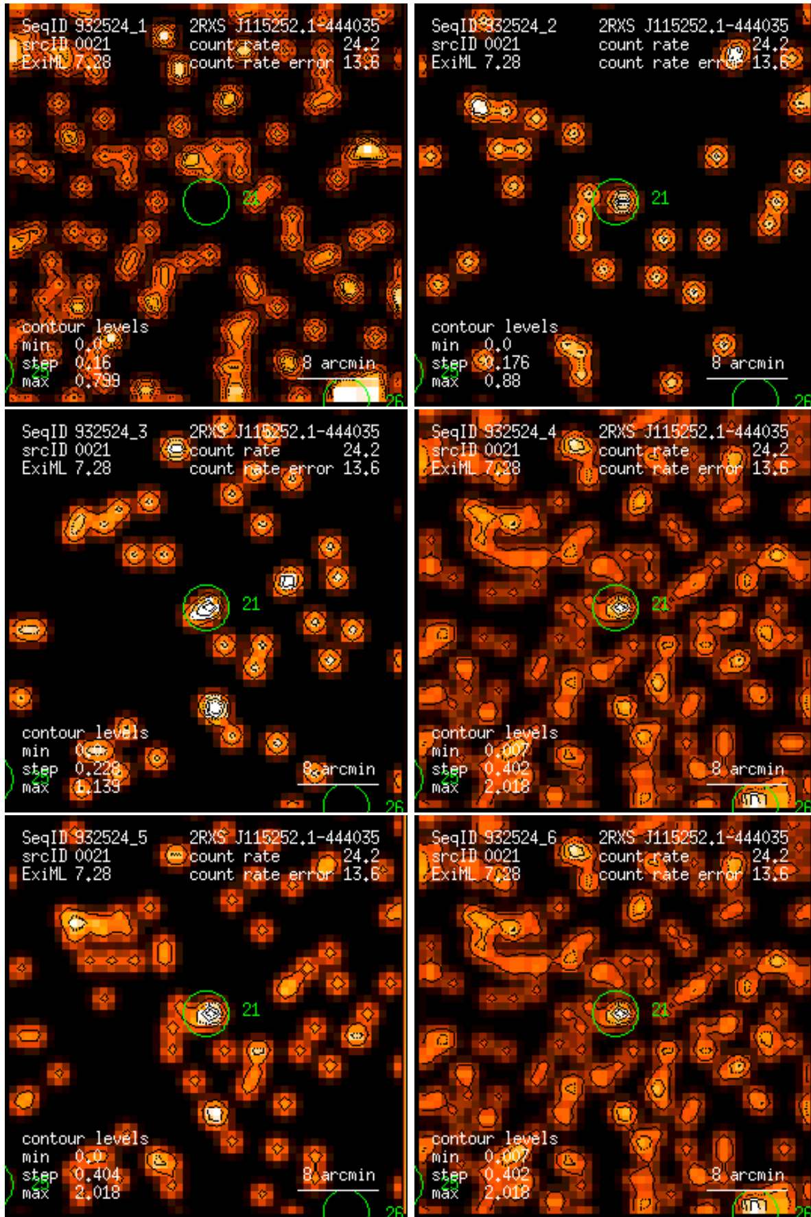
Figure 21: RASS 932524: detection 0021: band rate images, Gaussian filter: (1) PSPC channels 11 – 41, (2) 52 – 90, (3) 91 – 201, (4) 11 – 235, (5) 52 – 201, (6) 11 – 201. Broad band rates in counts/ks. Band rate contour levels in counts/ks/arcmin 2 .
