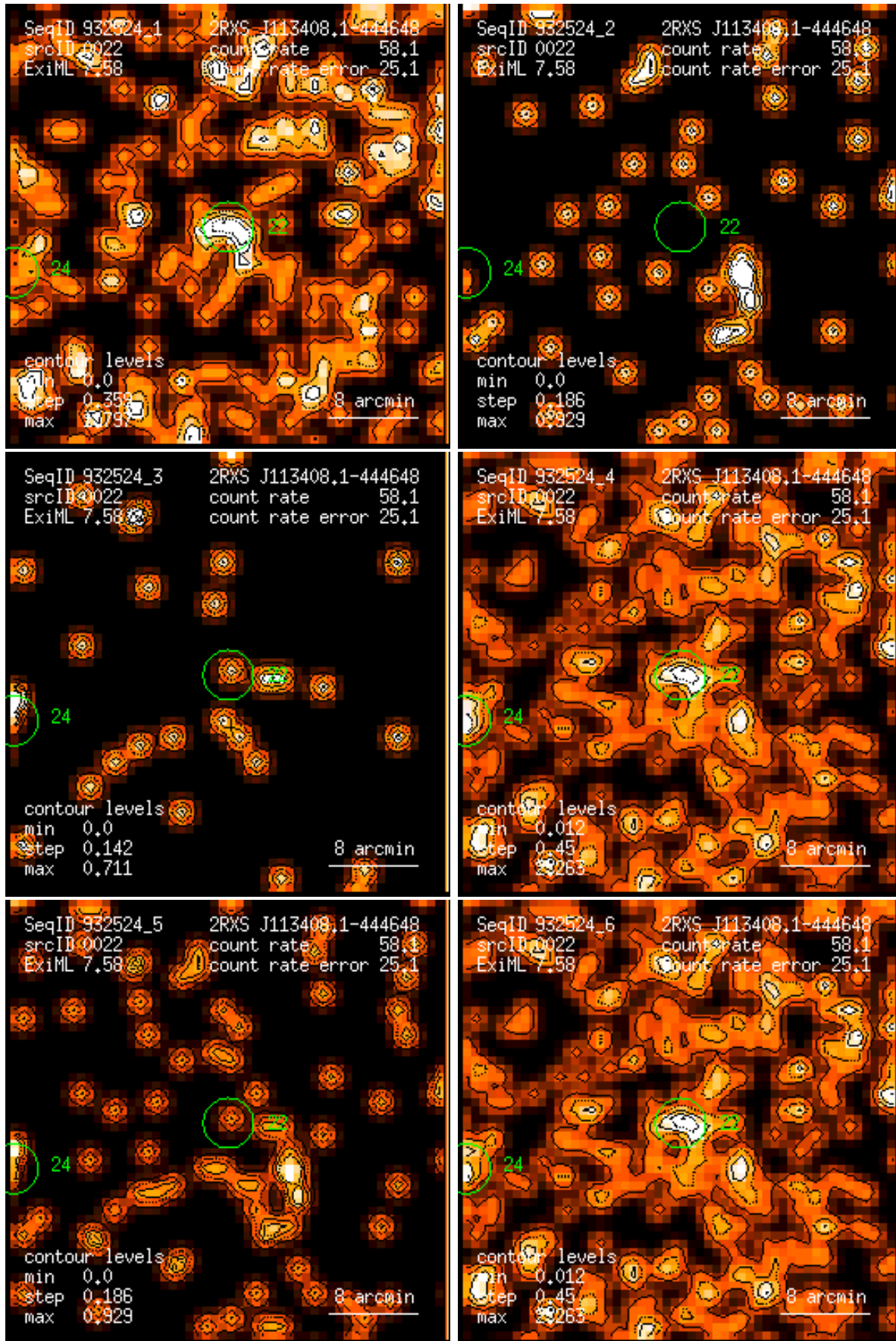
Figure 22: RASS 932524: detection 0022: band rate images, Gaussian filter: (1) PSPC channels 11 – 41, (2) 52 – 90, (3) 91 – 201, (4) 11 – 235, (5) 52 – 201, (6) 11 – 201. Broad band rates in counts/ks. Band rate contour levels in counts/ks/arcmin 2 .
