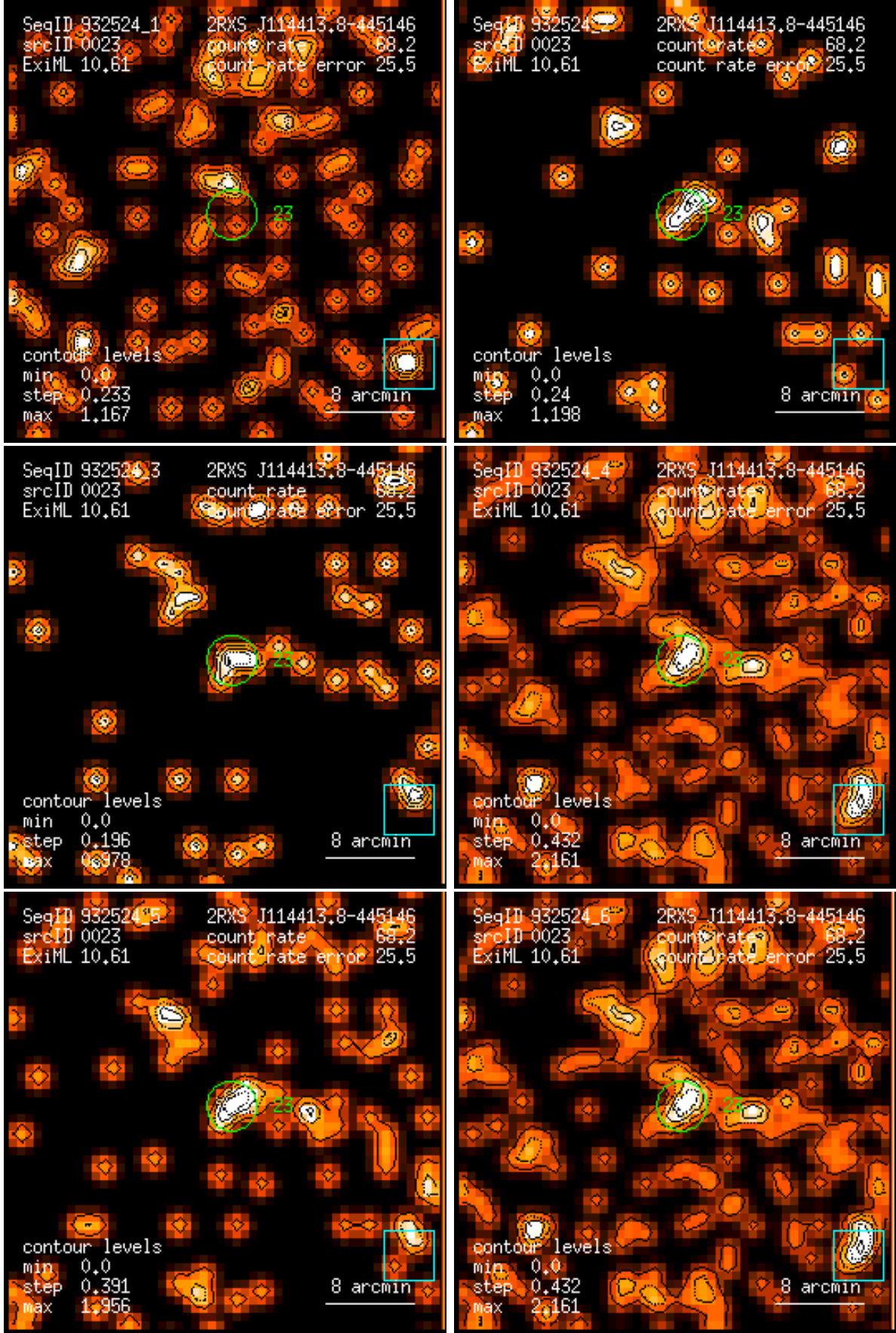
Figure 23: RASS 932524: detection 0023: band rate images, Gaussian filter: (1) PSPC channels 11 – 41, (2) 52 – 90, (3) 91 – 201, (4) 11 – 235, (5) 52 – 201, (6) 11 – 201. Broad band rates in counts/ks. Band rate contour levels in counts/ks/arcmin 2 .
