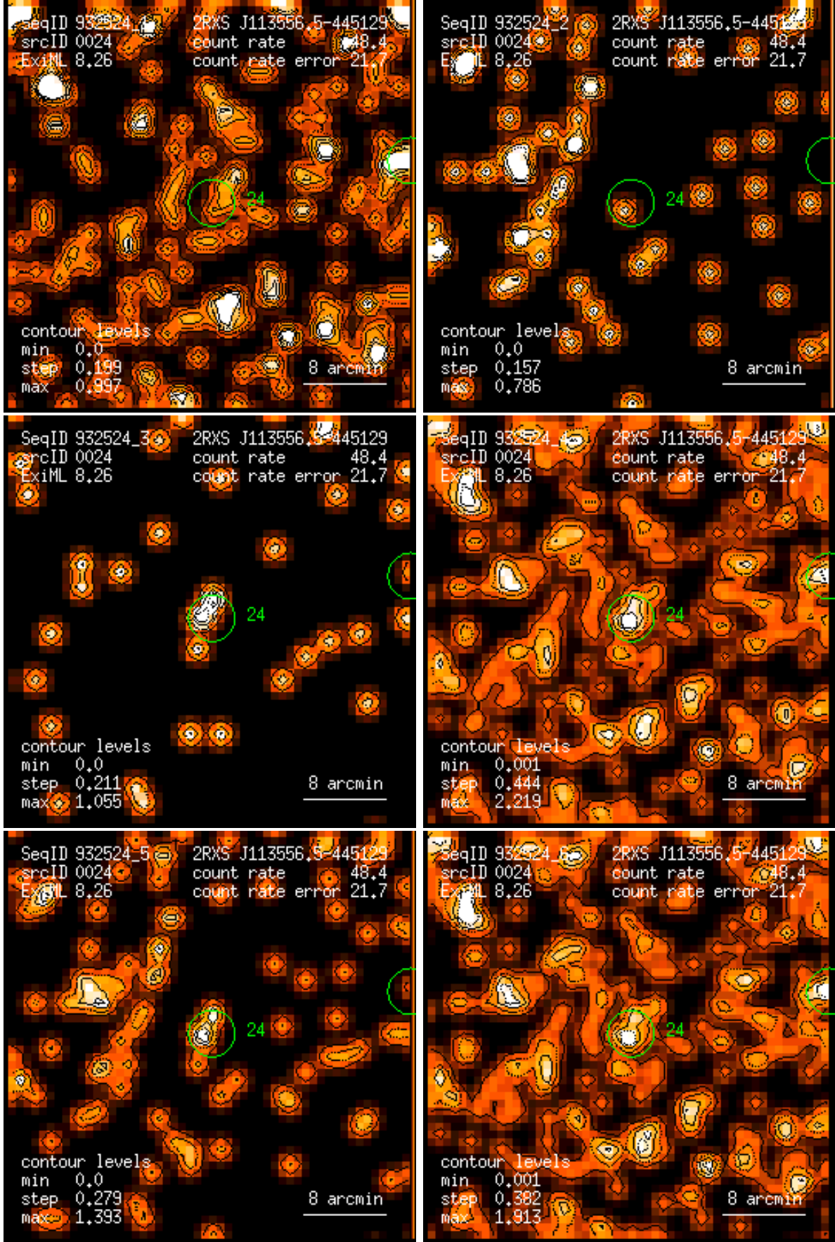
Figure 24: RASS 932524: detection 0024: band rate images, Gaussian filter: (1) PSPC channels 11 – 41, (2) 52 – 90, (3) 91 – 201, (4) 11 – 235, (5) 52 – 201, (6) 11 – 201. Broad band rates in counts/ks. Band rate contour levels in counts/ks/arcmin 2 .
