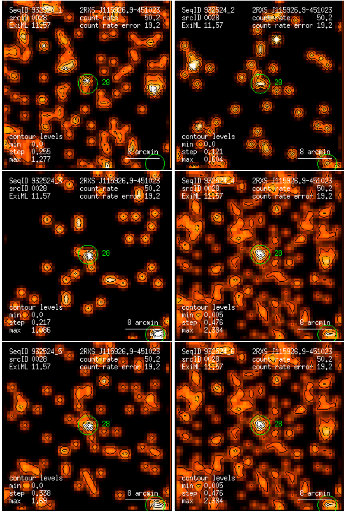
Figure 28: RASS 932524: detection 0028: band rate images, Gaussian filter: (1) PSPC channels 11 – 41, (2) 52 – 90, (3) 91 – 201, (4) 11 – 235, (5) 52 – 201, (6) 11 – 201. Broad band rates in counts/ks. Band rate contour levels in counts/ks/arcmin 2 .
