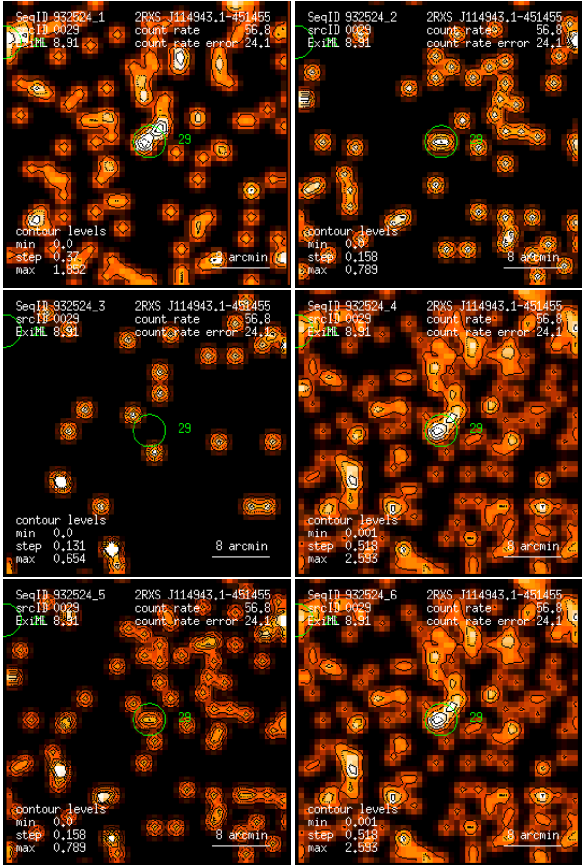
Figure 29: RASS 932524: detection 0029: band rate images, Gaussian filter: (1) PSPC channels 11 – 41, (2) 52 – 90, (3) 91 – 201, (4) 11 – 235, (5) 52 – 201, (6) 11 – 201. Broad band rates in counts/ks. Band rate contour levels in counts/ks/arcmin 2 .
