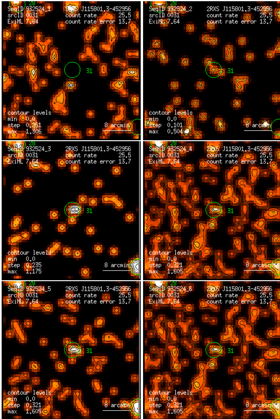
Figure 31: RASS 932524: detection 0031: band rate images, Gaussian filter: (1) PSPC channels 11 – 41, (2) 52 – 90, (3) 91 – 201, (4) 11 – 235, (5) 52 – 201, (6) 11 – 201. Broad band rates in counts/ks. Band rate contour levels in counts/ks/arcmin 2 .
