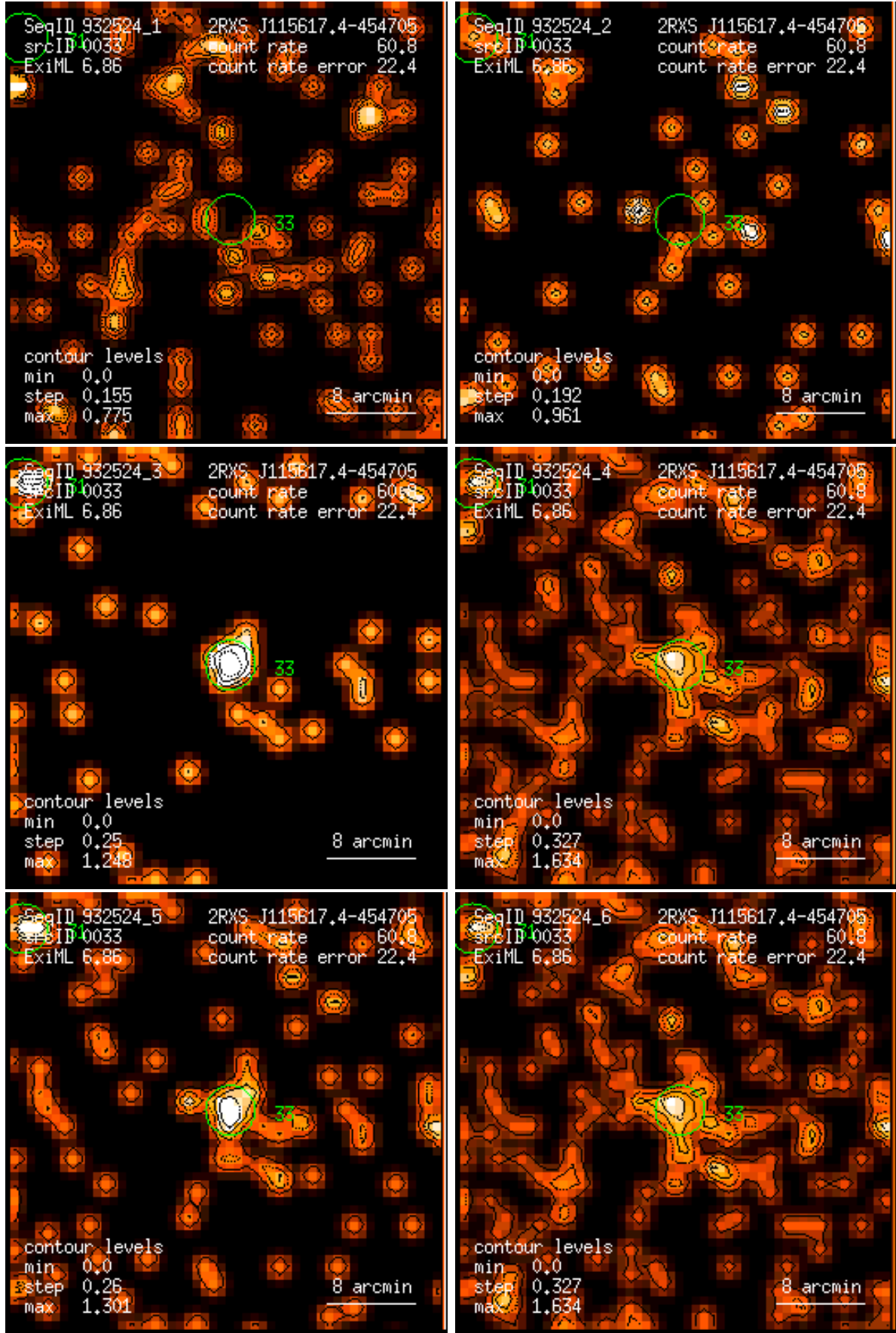
Figure 33: RASS 932524: detection 0033: band rate images, Gaussian filter: (1) PSPC channels 11 – 41, (2) 52 – 90, (3) 91 – 201, (4) 11 – 235, (5) 52 – 201, (6) 11 – 201. Broad band rates in counts/ks. Band rate contour levels in counts/ks/arcmin 2 .
