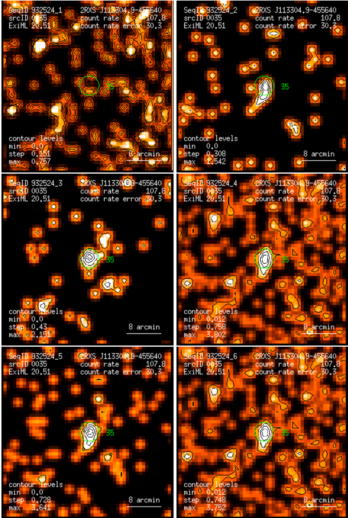
Figure 35: RASS 932524: detection 0035: band rate images, Gaussian filter: (1) PSPC channels 11 – 41, (2) 52 – 90, (3) 91 – 201, (4) 11 – 235, (5) 52 – 201, (6) 11 – 201. Broad band rates in counts/ks. Band rate contour levels in counts/ks/arcmin 2 .
