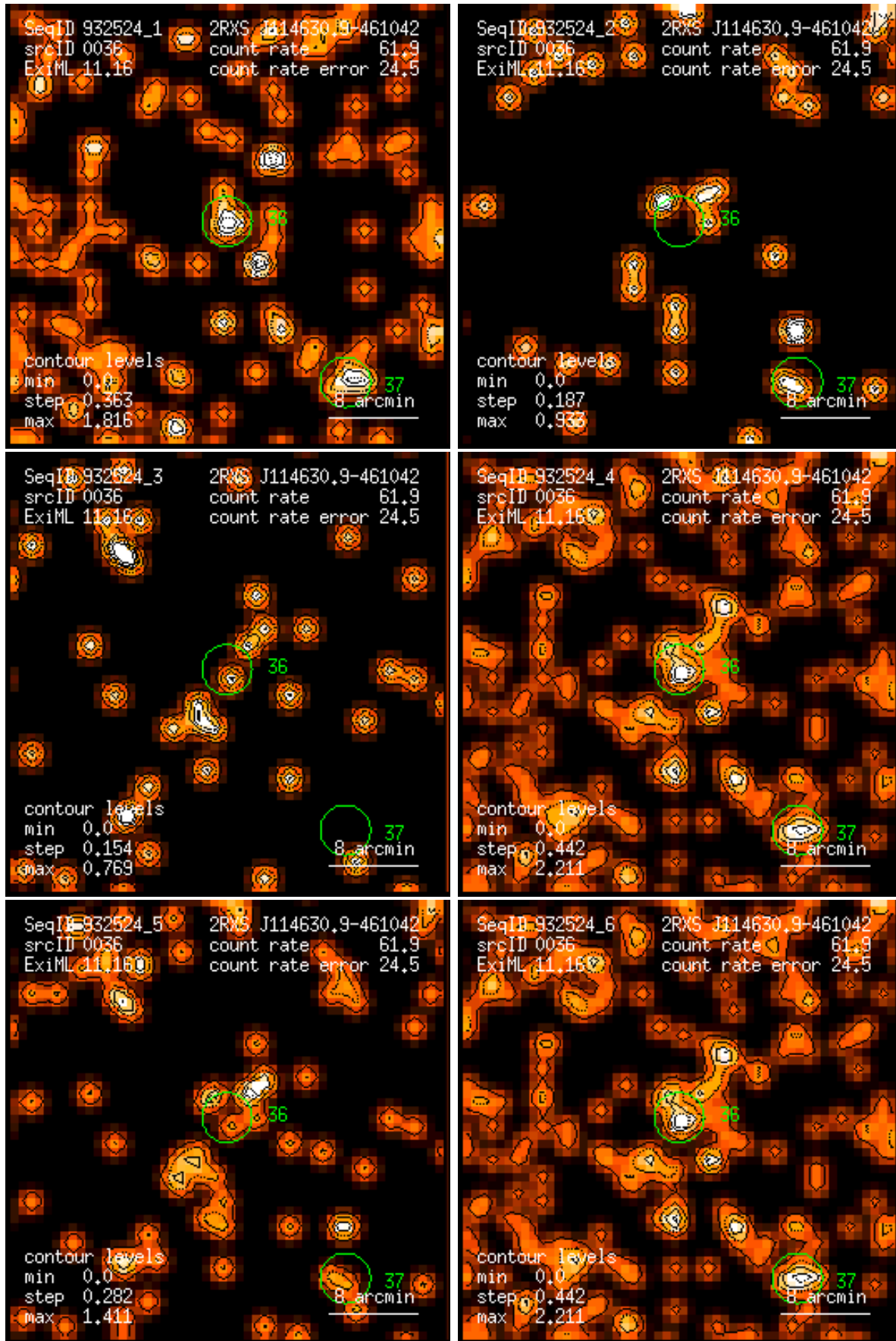
Figure 36: RASS 932524: detection 0036: band rate images, Gaussian filter: (1) PSPC channels 11 – 41, (2) 52 – 90, (3) 91 – 201, (4) 11 – 235, (5) 52 – 201, (6) 11 – 201. Broad band rates in counts/ks. Band rate contour levels in counts/ks/arcmin 2 .
