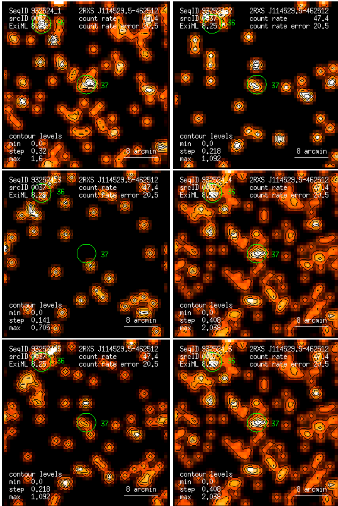
Figure 37: RASS 932524: detection 0037: band rate images, Gaussian filter: (1) PSPC channels 11 – 41, (2) 52 – 90, (3) 91 – 201, (4) 11 – 235, (5) 52 – 201, (6) 11 – 201. Broad band rates in counts/ks. Band rate contour levels in counts/ks/arcmin 2 .
