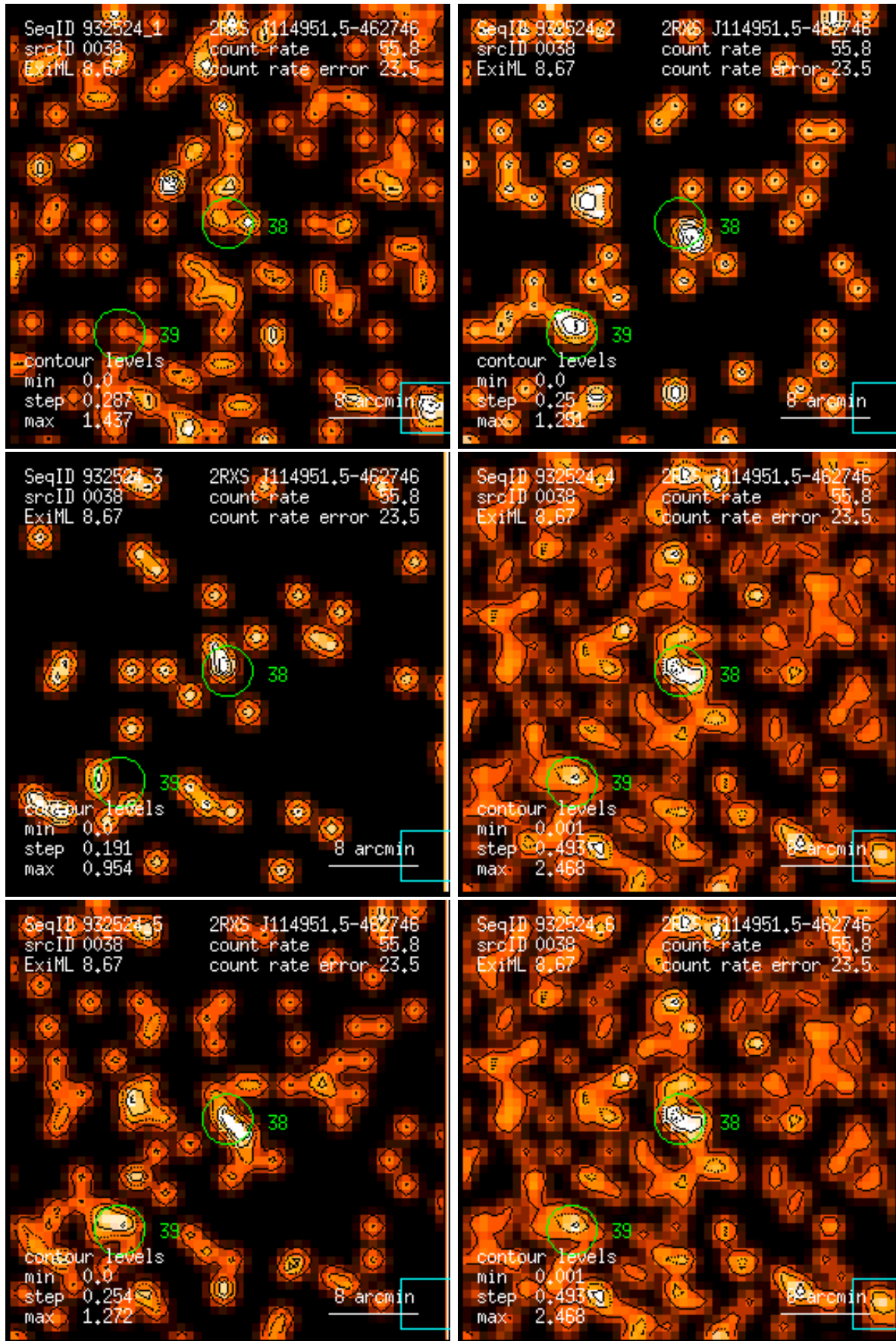
Figure 38: RASS 932524: detection 0038: band rate images, Gaussian filter: (1) PSPC channels 11 – 41, (2) 52 – 90, (3) 91 – 201, (4) 11 – 235, (5) 52 – 201, (6) 11 – 201. Broad band rates in counts/ks. Band rate contour levels in counts/ks/arcmin 2 .
