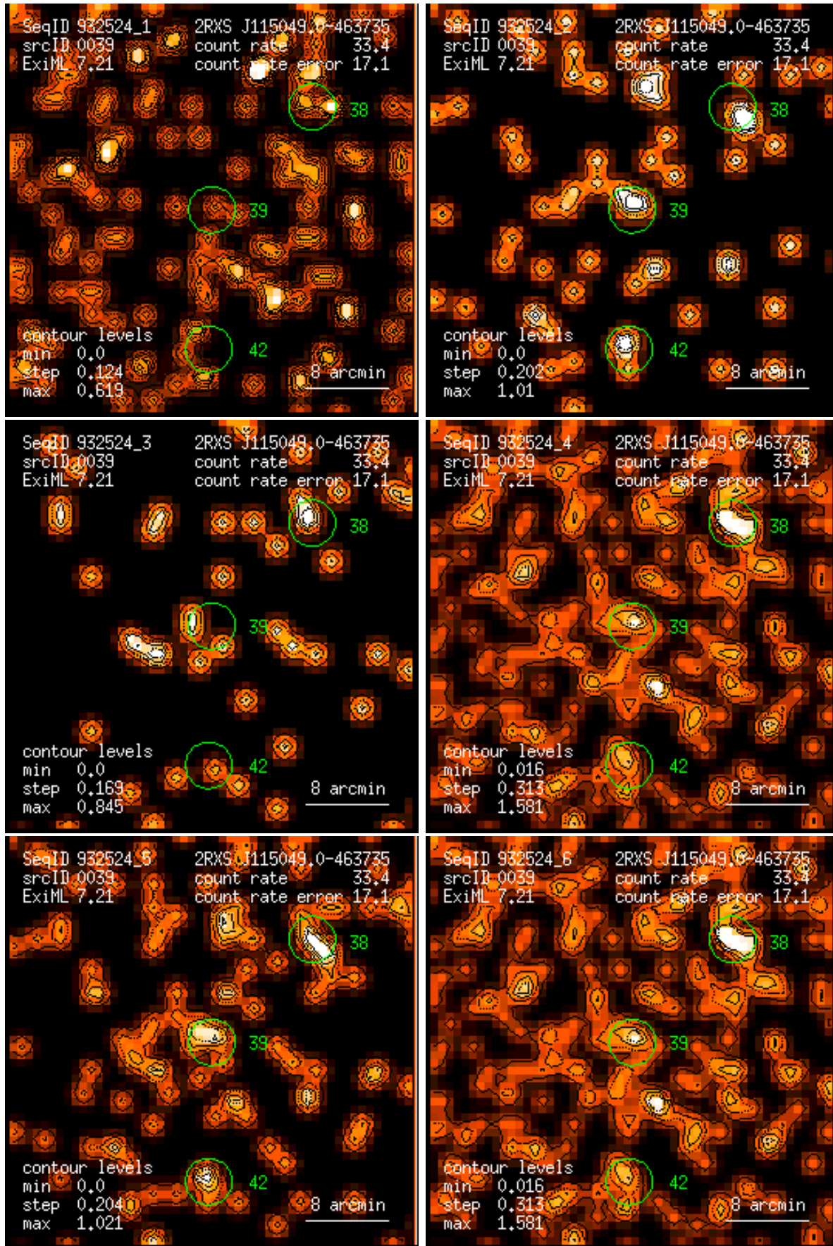
Figure 39: RASS 932524: detection 0039: band rate images, Gaussian filter: (1) PSPC channels 11 – 41, (2) 52 – 90, (3) 91 – 201, (4) 11 – 235, (5) 52 – 201, (6) 11 – 201. Broad band rates in counts/ks. Band rate contour levels in counts/ks/arcmin 2 .
