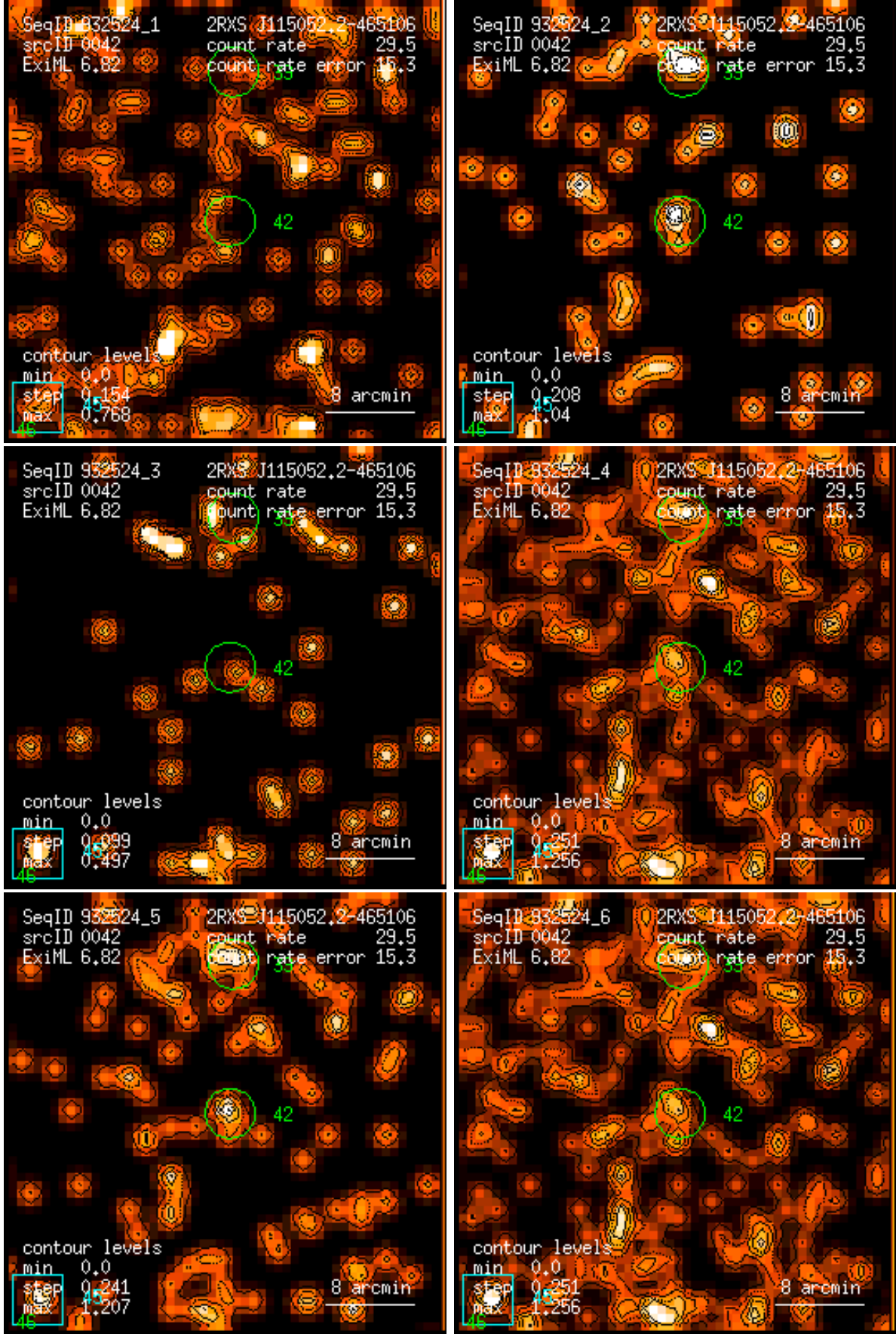
Figure 42: RASS 932524: detection 0042: band rate images, Gaussian filter: (1) PSPC channels 11 – 41, (2) 52 – 90, (3) 91 – 201, (4) 11 – 235, (5) 52 – 201, (6) 11 – 201. Broad band rates in counts/ks. Band rate contour levels in counts/ks/arcmin 2 .
