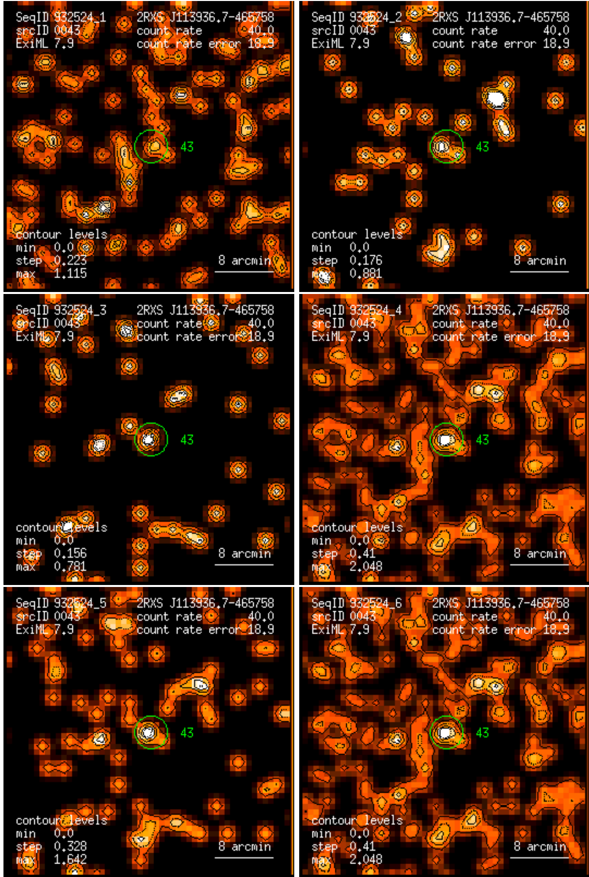
Figure 43: RASS 932524: detection 0043: band rate images, Gaussian filter: (1) PSPC channels 11 – 41, (2) 52 – 90, (3) 91 – 201, (4) 11 – 235, (5) 52 – 201, (6) 11 – 201. Broad band rates in counts/ks. Band rate contour levels in counts/ks/arcmin 2 .
