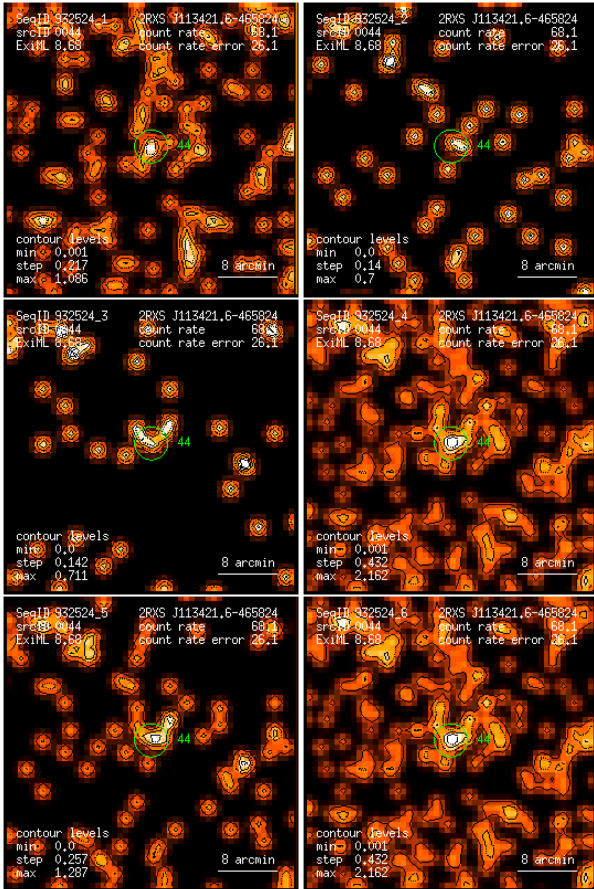
Figure 44: RASS 932524: detection 0044: band rate images, Gaussian filter: (1) PSPC channels 11 – 41, (2) 52 – 90, (3) 91 – 201, (4) 11 – 235, (5) 52 – 201, (6) 11 – 201. Broad band rates in counts/ks. Band rate contour levels in counts/ks/arcmin 2 .
