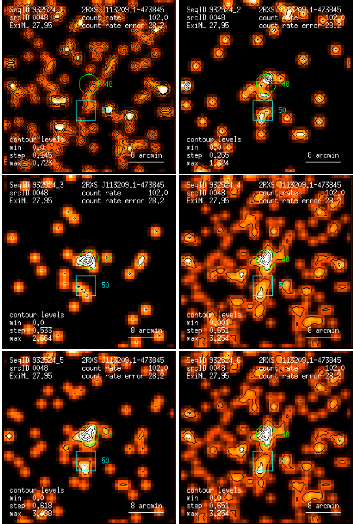
Figure 48: RASS 932524: detection 0048: band rate images, Gaussian filter: (1) PSPC channels 11 – 41, (2) 52 – 90, (3) 91 – 201, (4) 11 – 235, (5) 52 – 201, (6) 11 – 201. Broad band rates in counts/ks. Band rate contour levels in counts/ks/arcmin 2 .
