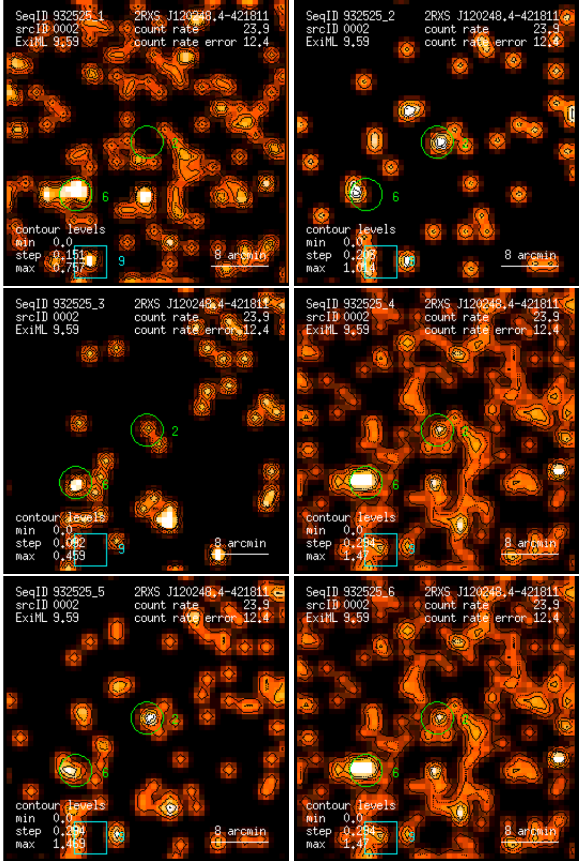
Figure 2: RASS 932525: detection 0002: band rate images, Gaussian filter: (1) PSPC channels 11 – 41, (2) 52 – 90, (3) 91 – 201, (4) 11 – 235, (5) 52 – 201, (6) 11 – 201. Broad band rates in counts/ks. Band rate contour levels in counts/ks/arcmin 2 .
