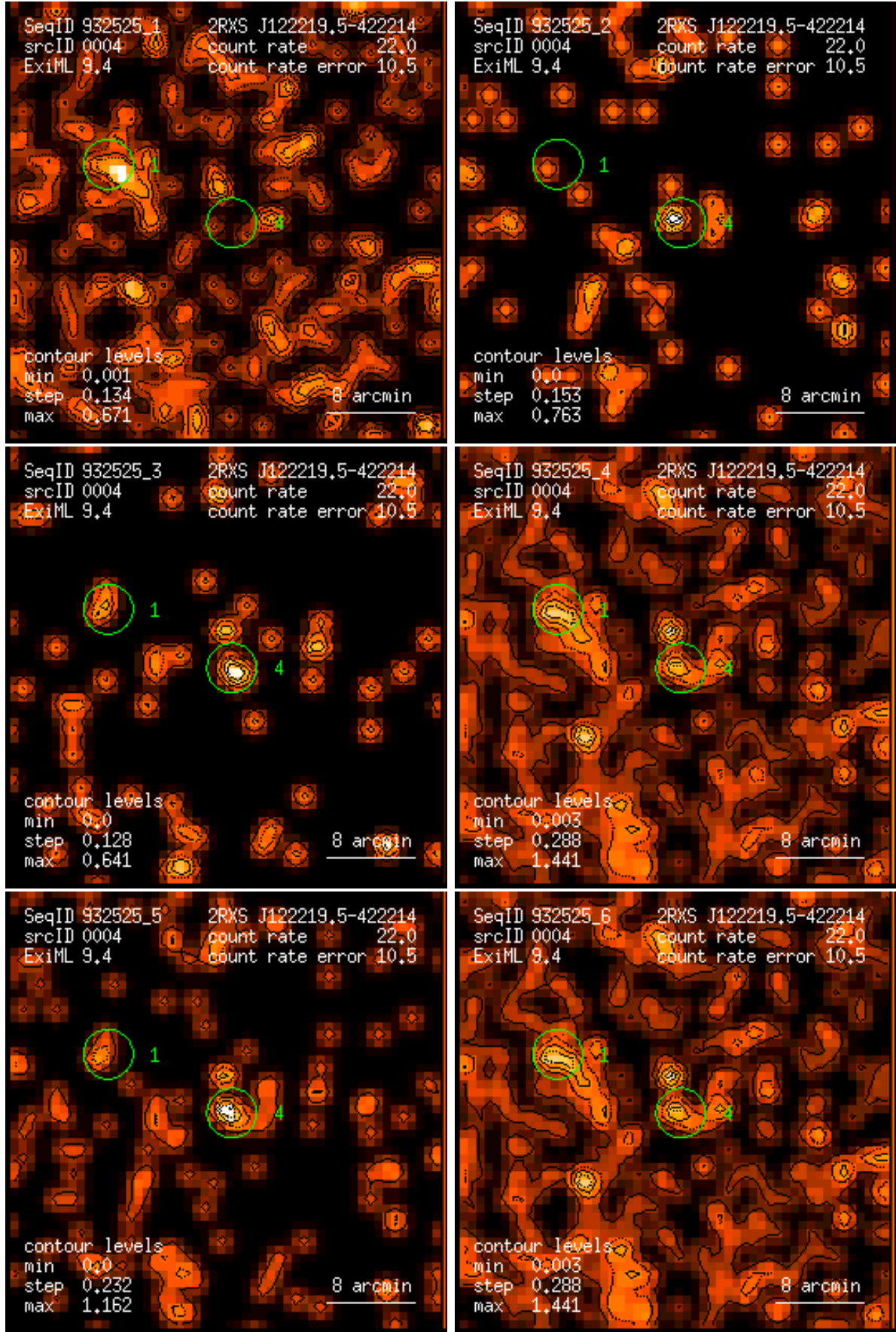
Figure 4: RASS 932525: detection 0004: band rate images, Gaussian filter: (1) PSPC channels 11 – 41, (2) 52 – 90, (3) 91 – 201, (4) 11 – 235, (5) 52 – 201, (6) 11 – 201. Broad band rates in counts/ks. Band rate contour levels in counts/ks/arcmin 2 .
