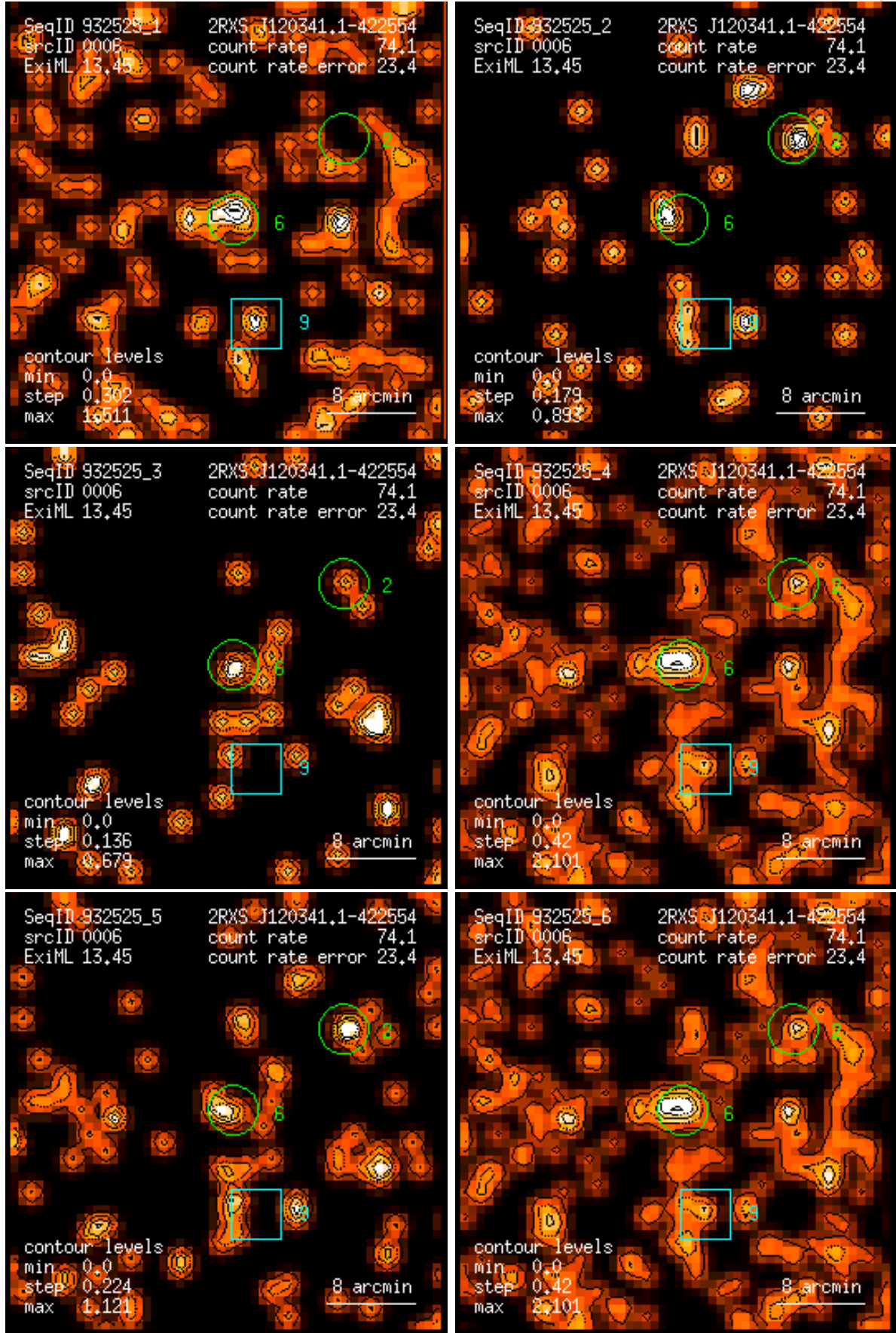
Figure 6: RASS 932525: detection 0006: band rate images, Gaussian filter: (1) PSPC channels 11 – 41, (2) 52 – 90, (3) 91 – 201, (4) 11 – 235, (5) 52 – 201, (6) 11 – 201. Broad band rates in counts/ks. Band rate contour levels in counts/ks/arcmin 2 .
