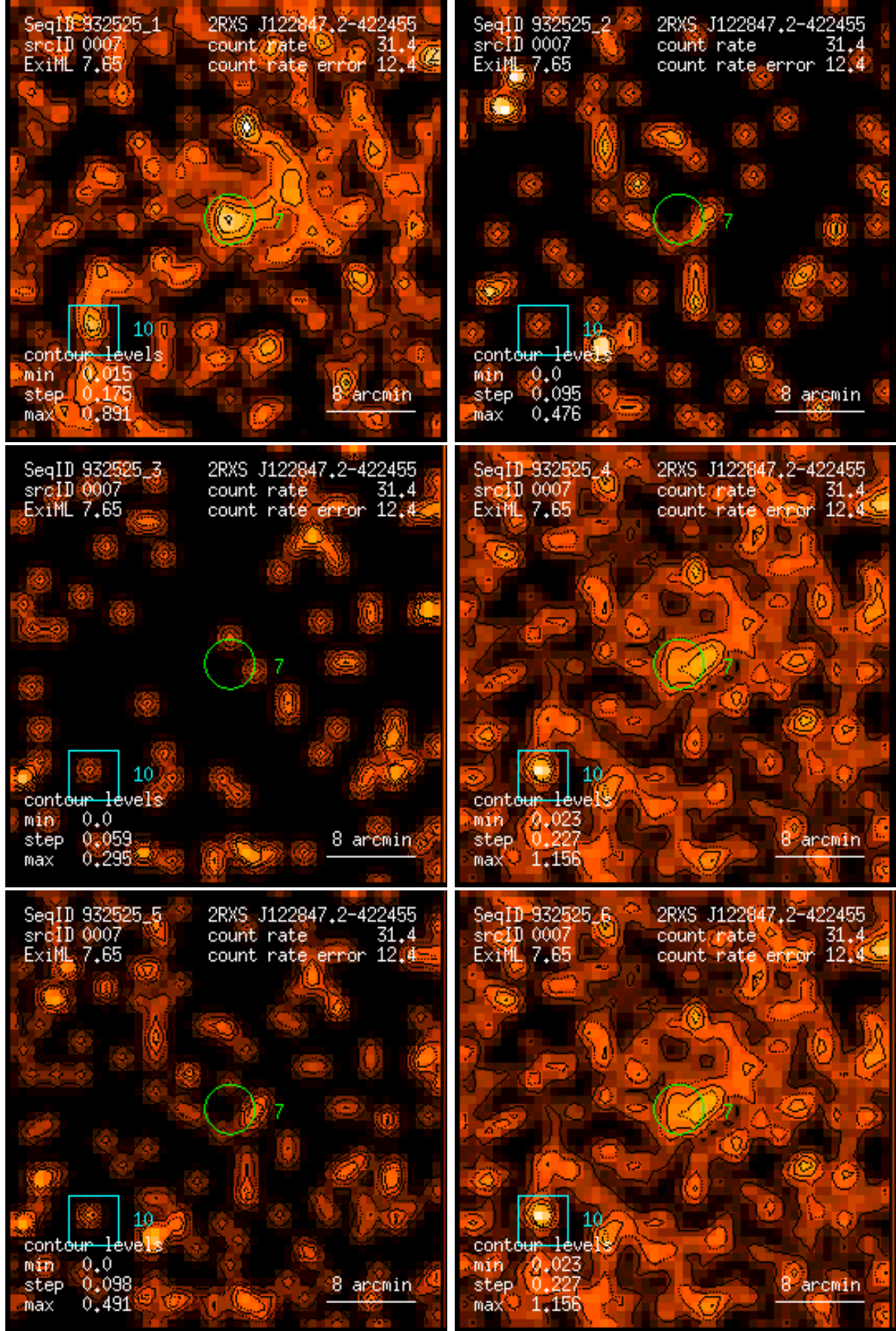
Figure 7: RASS 932525: detection 0007: band rate images, Gaussian filter: (1) PSPC channels 11 – 41, (2) 52 – 90, (3) 91 – 201, (4) 11 – 235, (5) 52 – 201, (6) 11 – 201. Broad band rates in counts/ks. Band rate contour levels in counts/ks/arcmin 2 .
