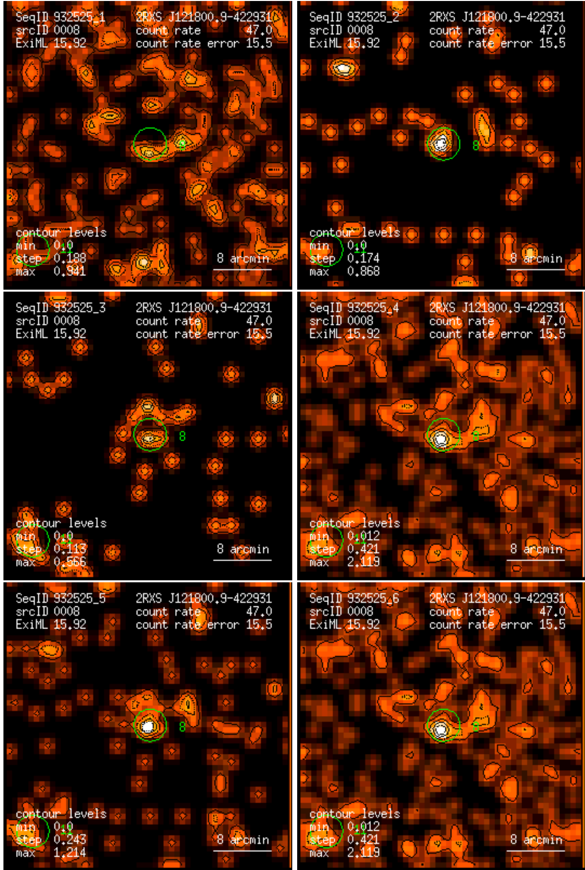
Figure 8: RASS 932525: detection 0008: band rate images, Gaussian filter: (1) PSPC channels 11 – 41, (2) 52 – 90, (3) 91 – 201, (4) 11 – 235, (5) 52 – 201, (6) 11 – 201. Broad band rates in counts/ks. Band rate contour levels in counts/ks/arcmin 2 .
