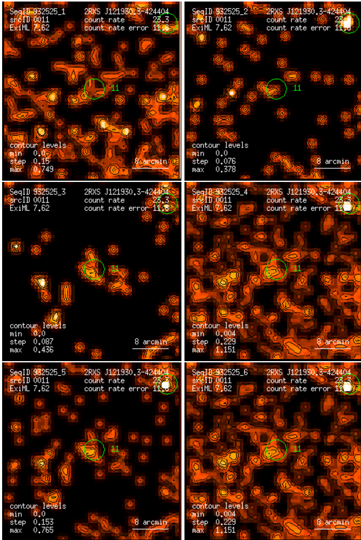
Figure 11: RASS 932525: detection 0011: band rate images, Gaussian filter: (1) PSPC channels 11 – 41, (2) 52 – 90, (3) 91 – 201, (4) 11 – 235, (5) 52 – 201, (6) 11 – 201. Broad band rates in counts/ks. Band rate contour levels in counts/ks/arcmin 2 .
