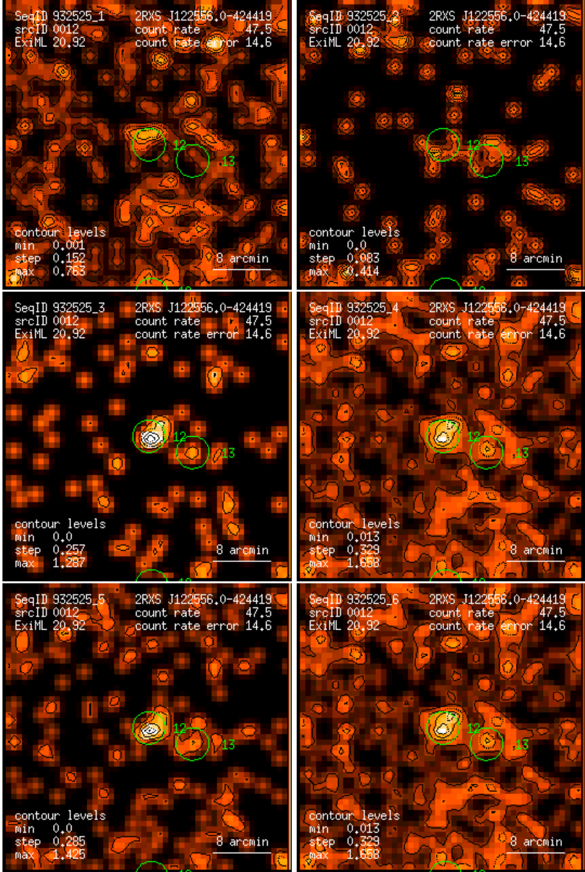
Figure 12: RASS 932525: detection 0012: band rate images, Gaussian filter: (1) PSPC channels 11 – 41, (2) 52 – 90, (3) 91 – 201, (4) 11 – 235, (5) 52 – 201, (6) 11 – 201. Broad band rates in counts/ks. Band rate contour levels in counts/ks/arcmin 2 .
