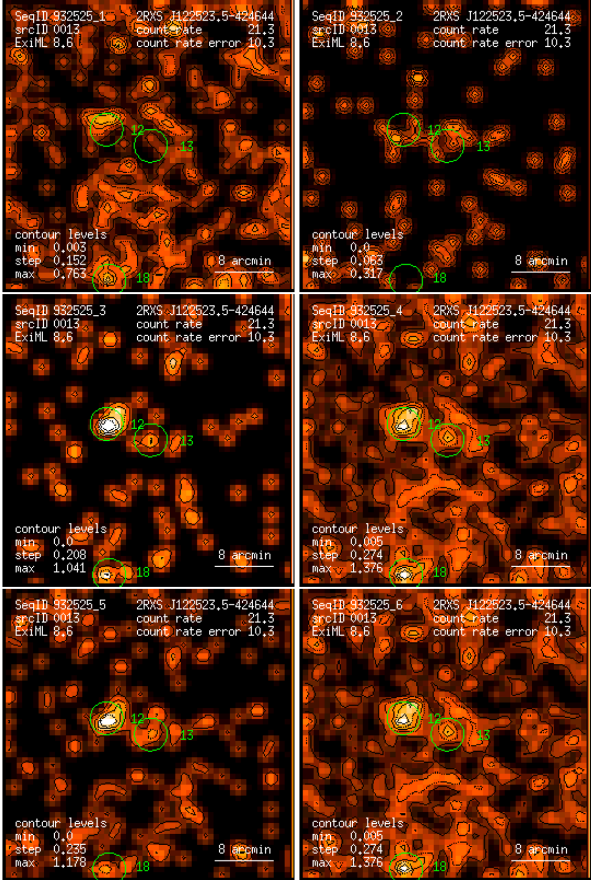
Figure 13: RASS 932525: detection 0013: band rate images, Gaussian filter: (1) PSPC channels 11 – 41, (2) 52 – 90, (3) 91 – 201, (4) 11 – 235, (5) 52 – 201, (6) 11 – 201. Broad band rates in counts/ks. Band rate contour levels in counts/ks/arcmin 2 .
