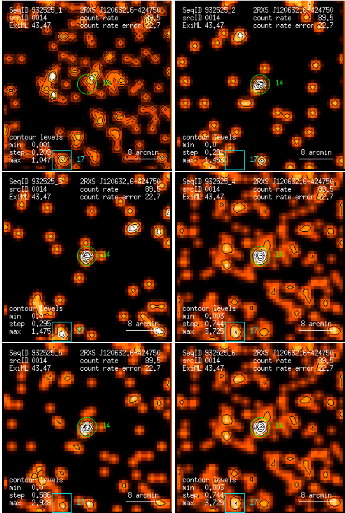
Figure 14: RASS 932525: detection 0014: band rate images, Gaussian filter: (1) PSPC channels 11 – 41, (2) 52 – 90, (3) 91 – 201, (4) 11 – 235, (5) 52 – 201, (6) 11 – 201. Broad band rates in counts/ks. Band rate contour levels in counts/ks/arcmin 2 .
