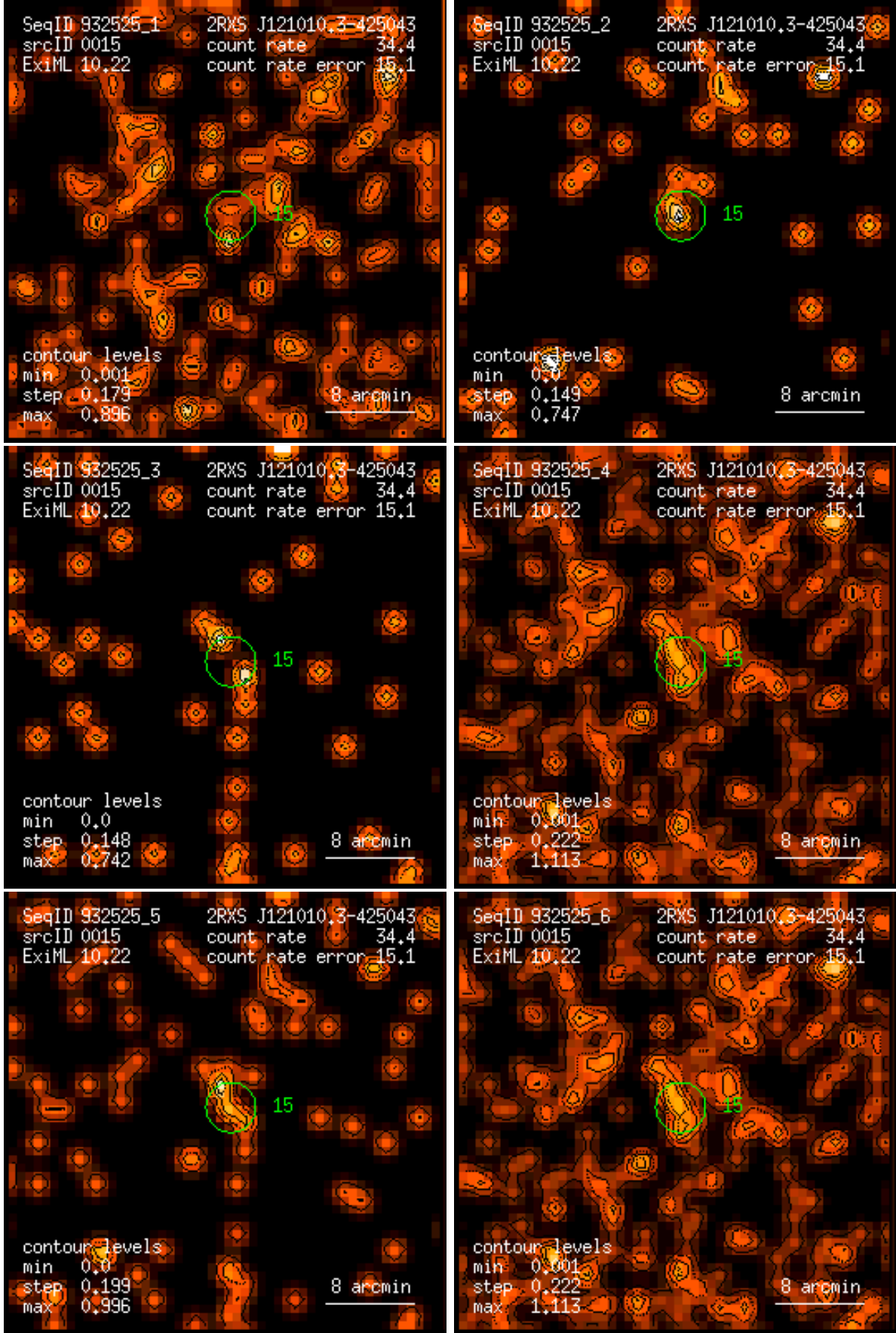
Figure 15: RASS 932525: detection 0015: band rate images, Gaussian filter: (1) PSPC channels 11 – 41, (2) 52 – 90, (3) 91 – 201, (4) 11 – 235, (5) 52 – 201, (6) 11 – 201. Broad band rates in counts/ks. Band rate contour levels in counts/ks/arcmin 2 .
