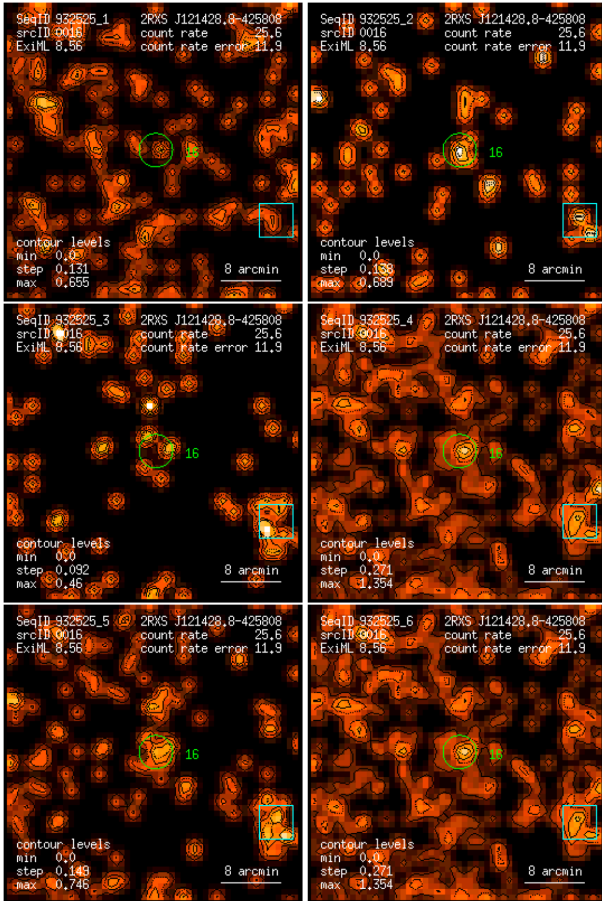
Figure 16: RASS 932525: detection 0016: band rate images, Gaussian filter: (1) PSPC channels 11 – 41, (2) 52 – 90, (3) 91 – 201, (4) 11 – 235, (5) 52 – 201, (6) 11 – 201. Broad band rates in counts/ks. Band rate contour levels in counts/ks/arcmin 2 .
