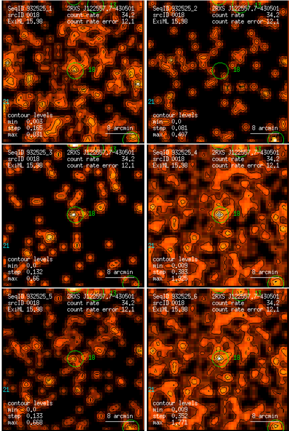
Figure 18: RASS 932525: detection 0018: band rate images, Gaussian filter: (1) PSPC channels 11 – 41, (2) 52 – 90, (3) 91 – 201, (4) 11 – 235, (5) 52 – 201, (6) 11 – 201. Broad band rates in counts/ks. Band rate contour levels in counts/ks/arcmin 2 .
