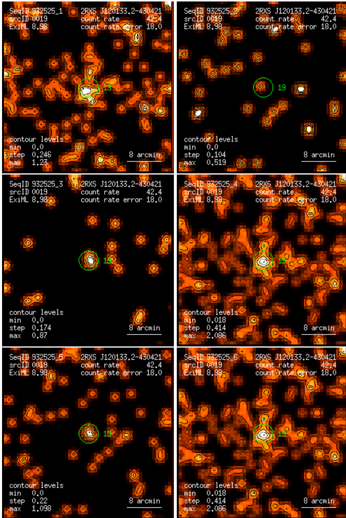
Figure 19: RASS 932525: detection 0019: band rate images, Gaussian filter: (1) PSPC channels 11 – 41, (2) 52 – 90, (3) 91 – 201, (4) 11 – 235, (5) 52 – 201, (6) 11 – 201. Broad band rates in counts/ks. Band rate contour levels in counts/ks/arcmin 2 .
