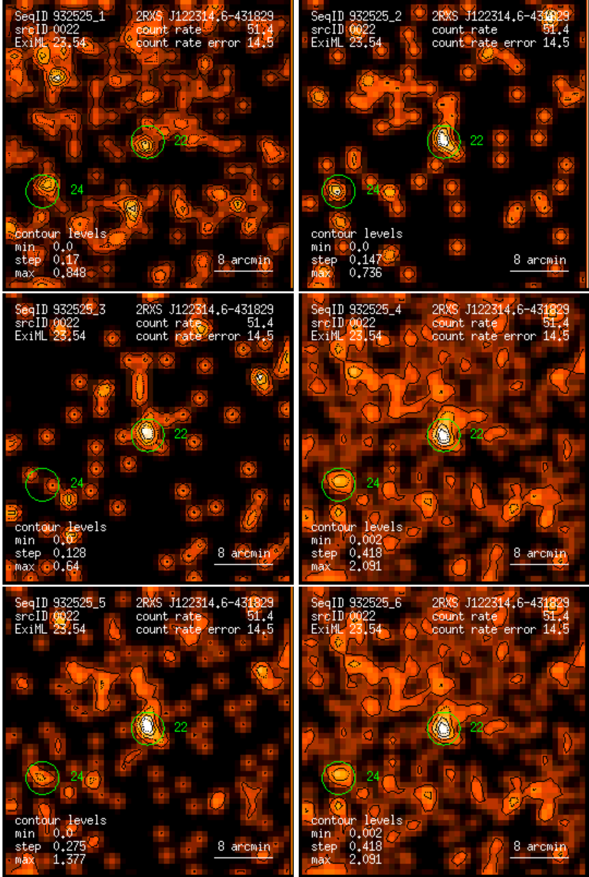
Figure 22: RASS 932525: detection 0022: band rate images, Gaussian filter: (1) PSPC channels 11 – 41, (2) 52 – 90, (3) 91 – 201, (4) 11 – 235, (5) 52 – 201, (6) 11 – 201. Broad band rates in counts/ks. Band rate contour levels in counts/ks/arcmin 2 .
