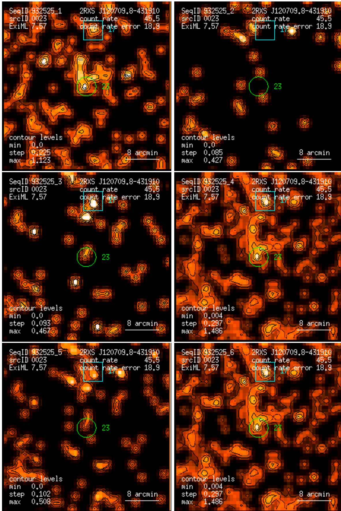
Figure 23: RASS 932525: detection 0023: band rate images, Gaussian filter: (1) PSPC channels 11 – 41, (2) 52 – 90, (3) 91 – 201, (4) 11 – 235, (5) 52 – 201, (6) 11 – 201. Broad band rates in counts/ks. Band rate contour levels in counts/ks/arcmin 2 .
