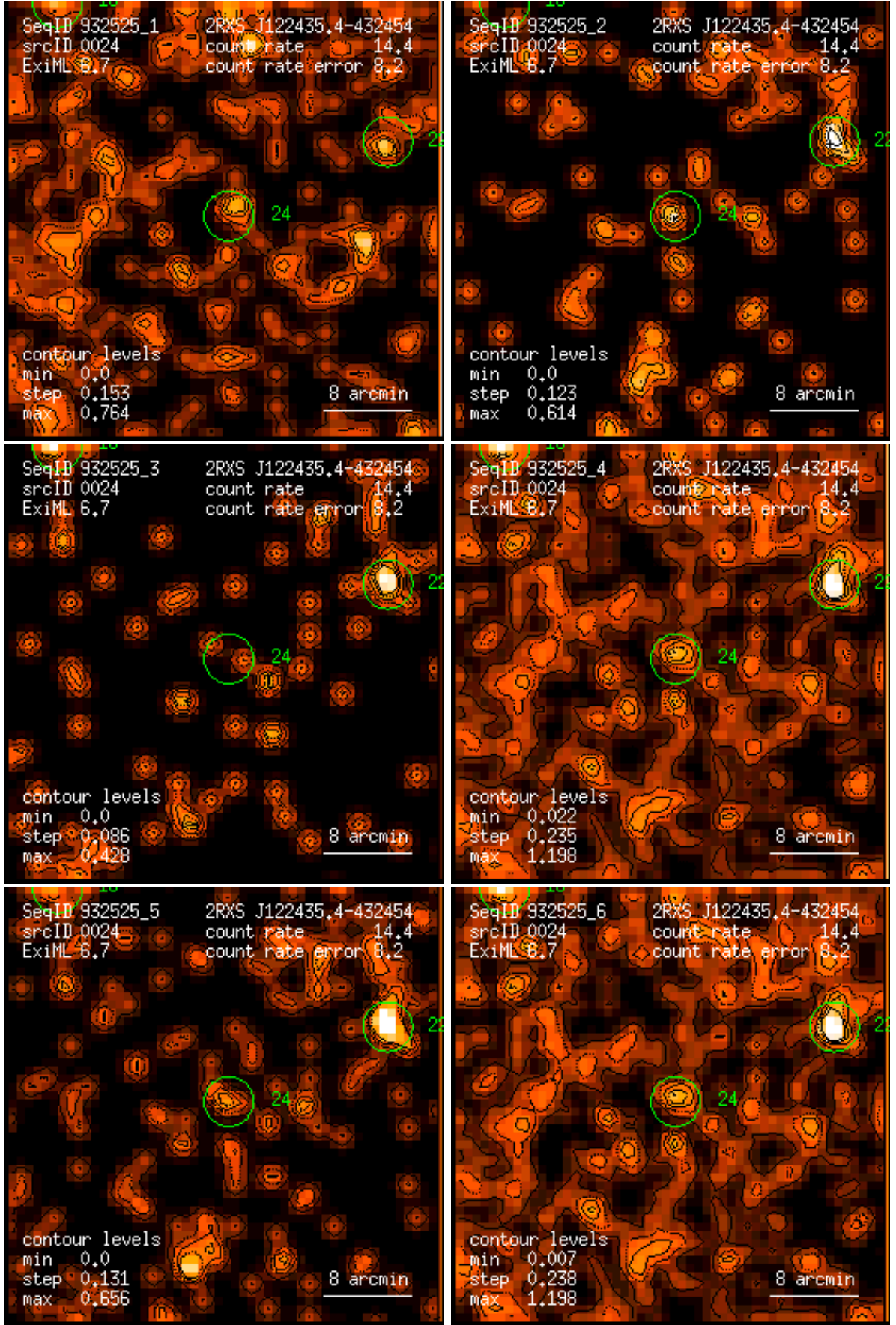
Figure 24: RASS 932525: detection 0024: band rate images, Gaussian filter: (1) PSPC channels 11 – 41, (2) 52 – 90, (3) 91 – 201, (4) 11 – 235, (5) 52 – 201, (6) 11 – 201. Broad band rates in counts/ks. Band rate contour levels in counts/ks/arcmin 2 .
