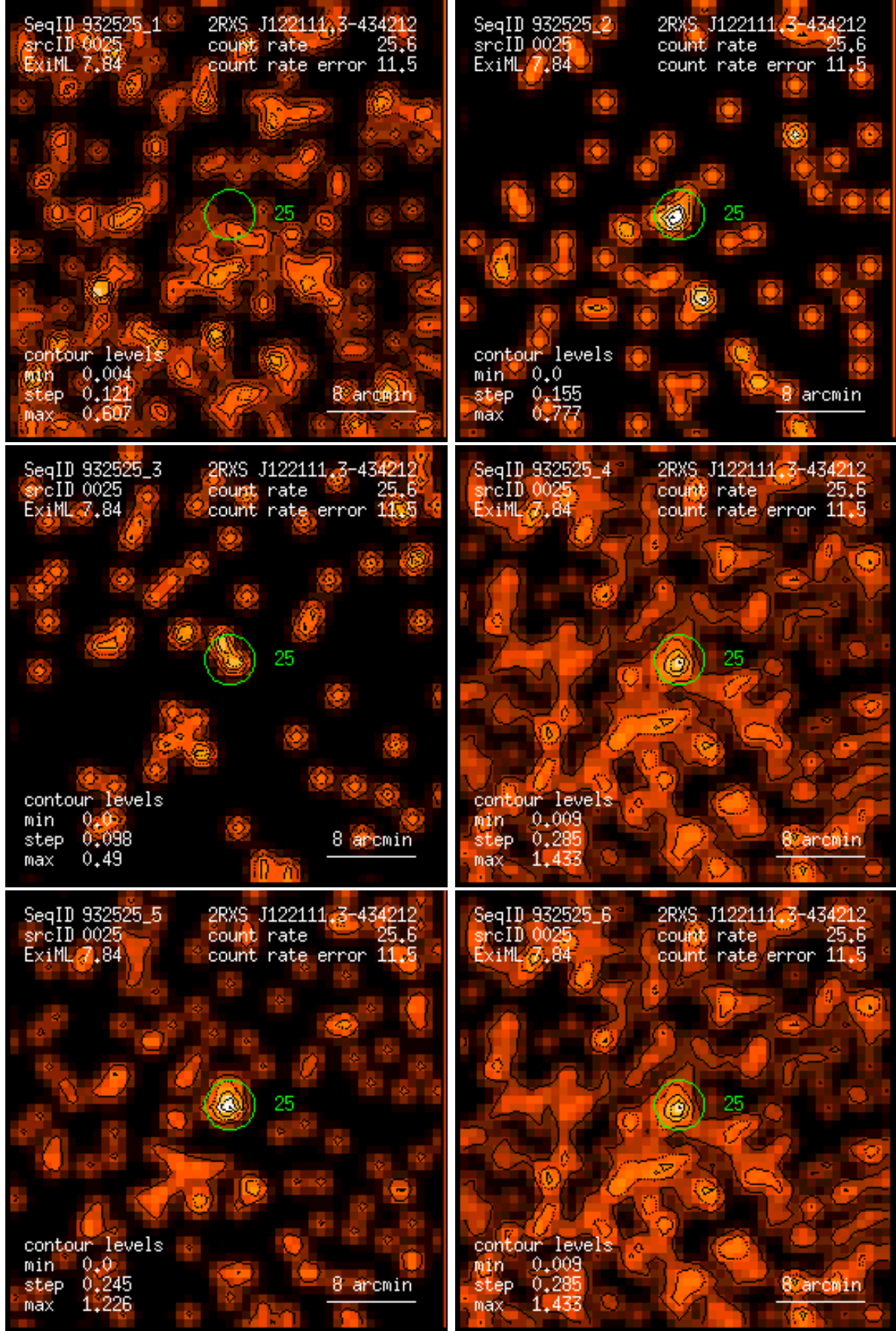
Figure 25: RASS 932525: detection 0025: band rate images, Gaussian filter: (1) PSPC channels 11 – 41, (2) 52 – 90, (3) 91 – 201, (4) 11 – 235, (5) 52 – 201, (6) 11 – 201. Broad band rates in counts/ks. Band rate contour levels in counts/ks/arcmin 2 .
