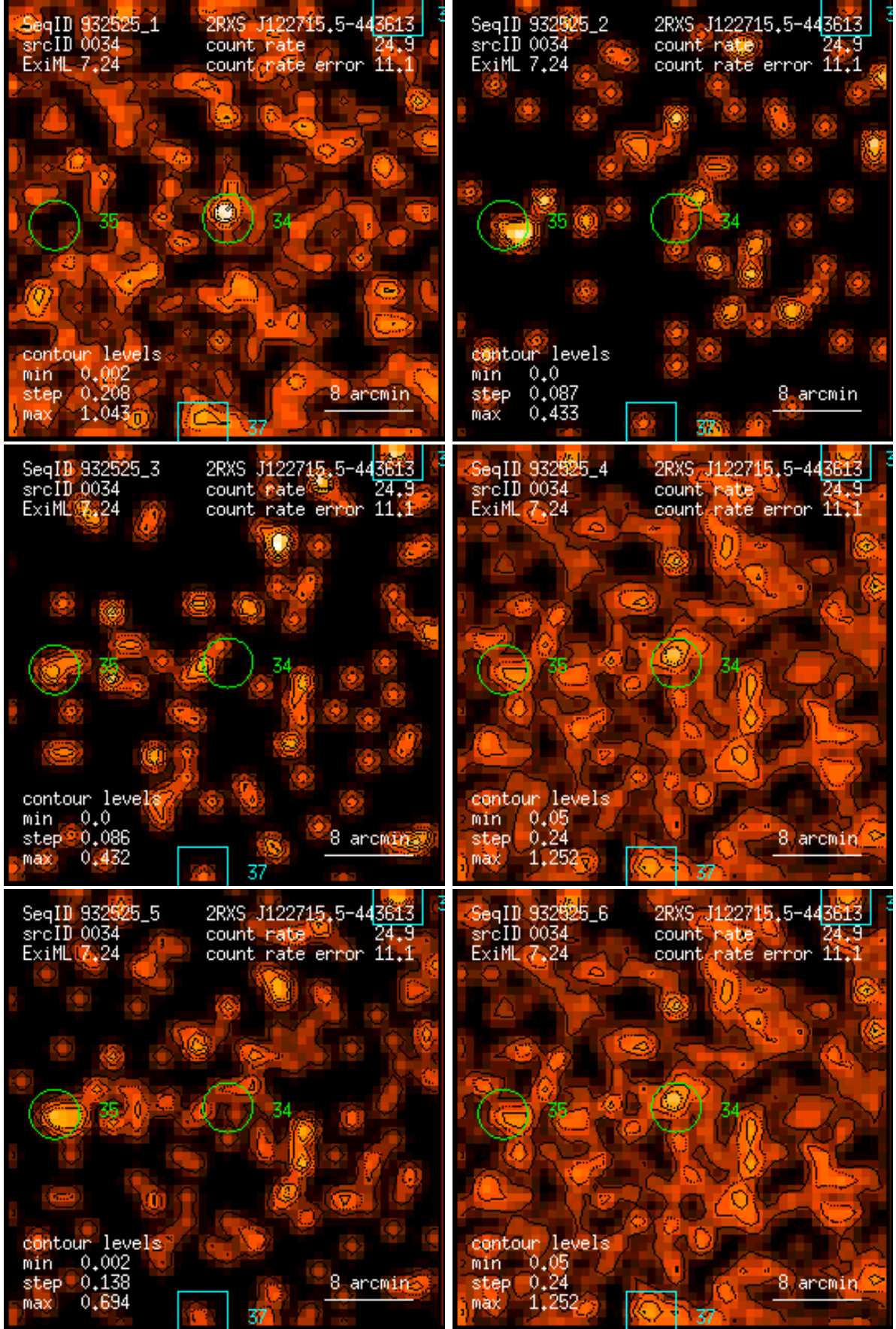
Figure 34: RASS 932525: detection 0034: band rate images, Gaussian filter: (1) PSPC channels 11 – 41, (2) 52 – 90, (3) 91 – 201, (4) 11 – 235, (5) 52 – 201, (6) 11 – 201. Broad band rates in counts/ks. Band rate contour levels in counts/ks/arcmin 2 .
