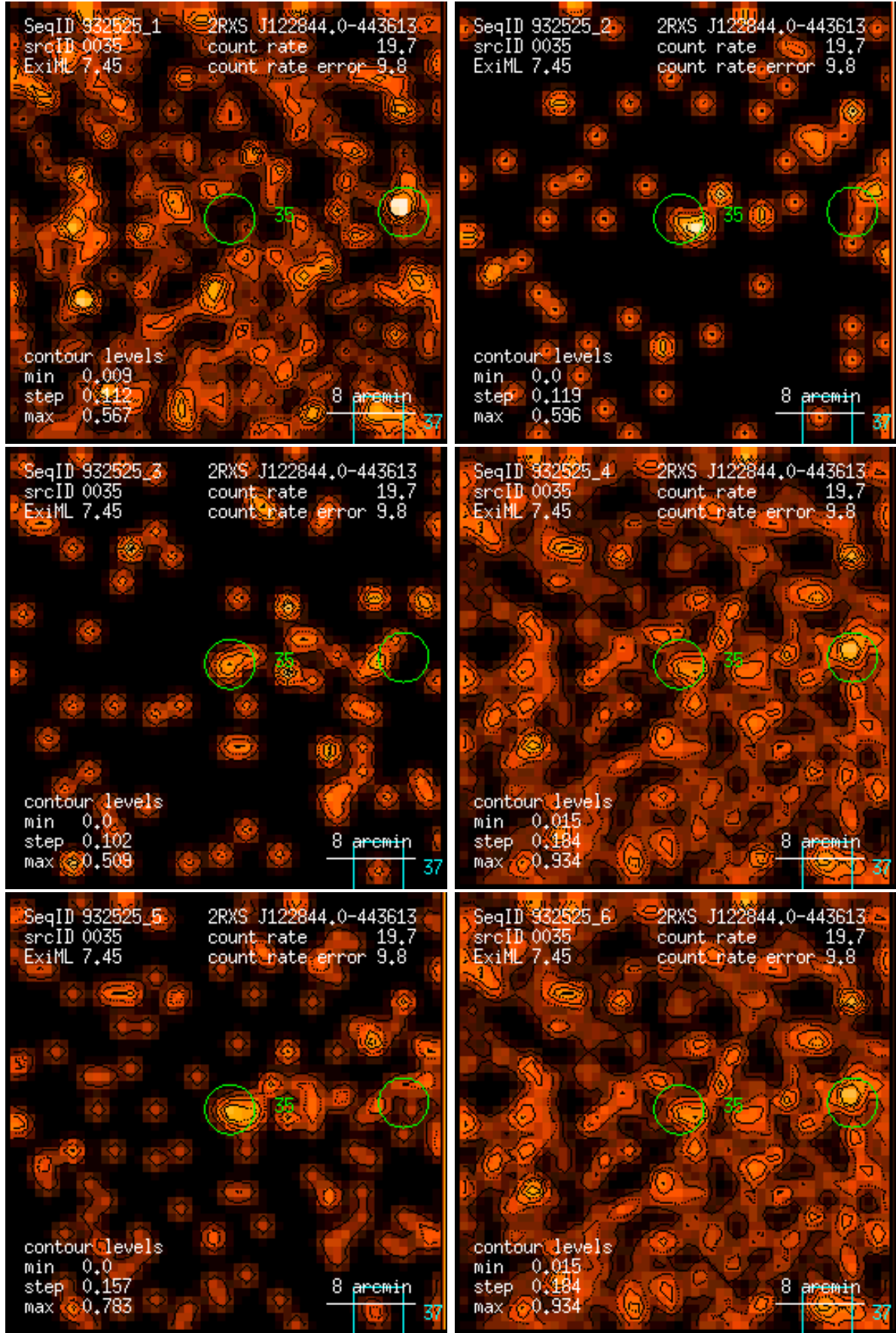
Figure 35: RASS 932525: detection 0035: band rate images, Gaussian filter: (1) PSPC channels 11 – 41, (2) 52 – 90, (3) 91 – 201, (4) 11 – 235, (5) 52 – 201, (6) 11 – 201. Broad band rates in counts/ks. Band rate contour levels in counts/ks/arcmin 2 .
