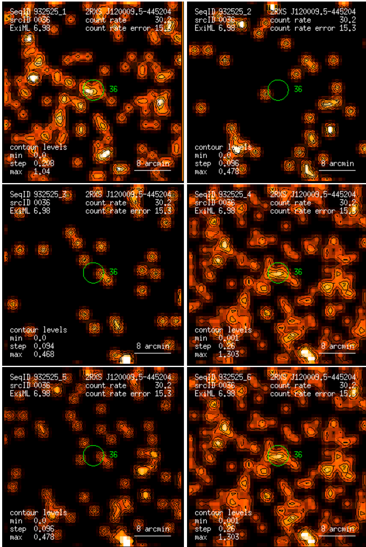
Figure 36: RASS 932525: detection 0036: band rate images, Gaussian filter: (1) PSPC channels 11 – 41, (2) 52 – 90, (3) 91 – 201, (4) 11 – 235, (5) 52 – 201, (6) 11 – 201. Broad band rates in counts/ks. Band rate contour levels in counts/ks/arcmin 2 .
