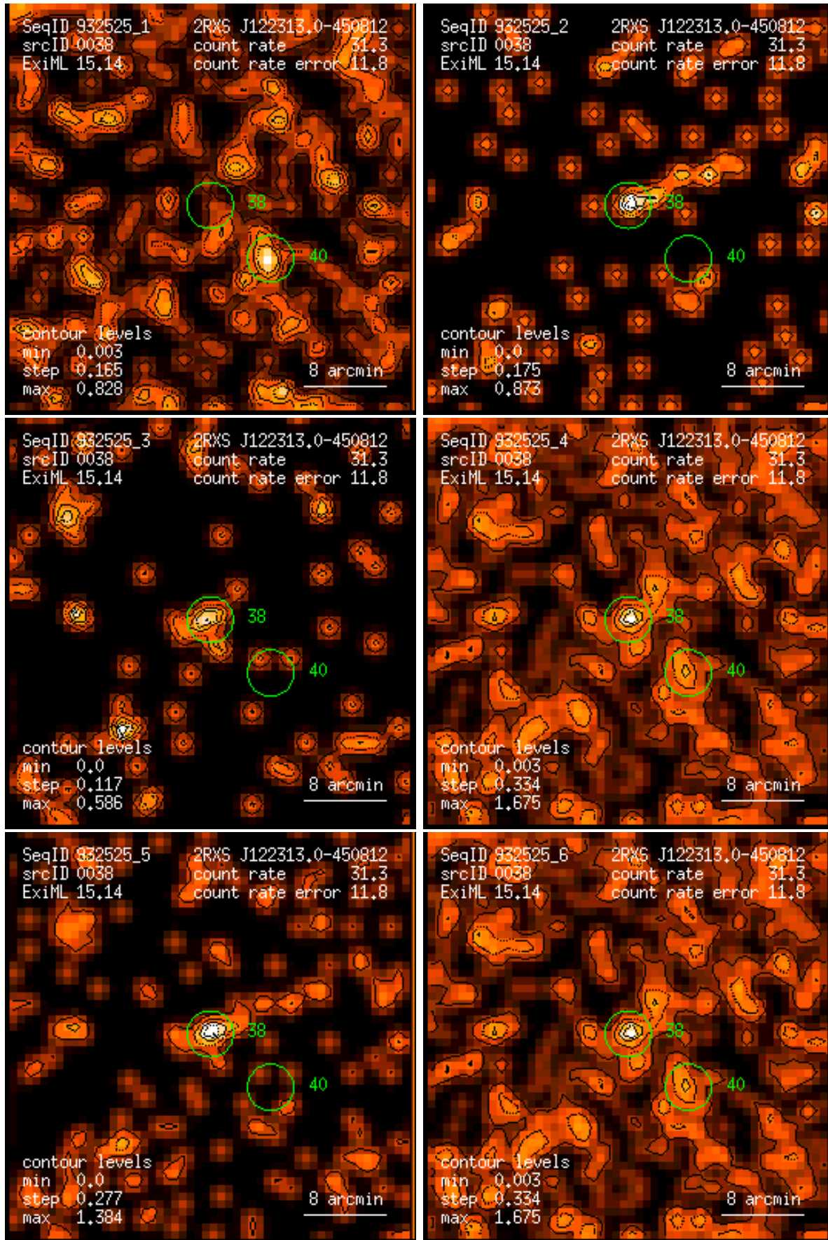
Figure 38: RASS 932525: detection 0038: band rate images, Gaussian filter: (1) PSPC channels 11 – 41, (2) 52 – 90, (3) 91 – 201, (4) 11 – 235, (5) 52 – 201, (6) 11 – 201. Broad band rates in counts/ks. Band rate contour levels in counts/ks/arcmin 2 .
