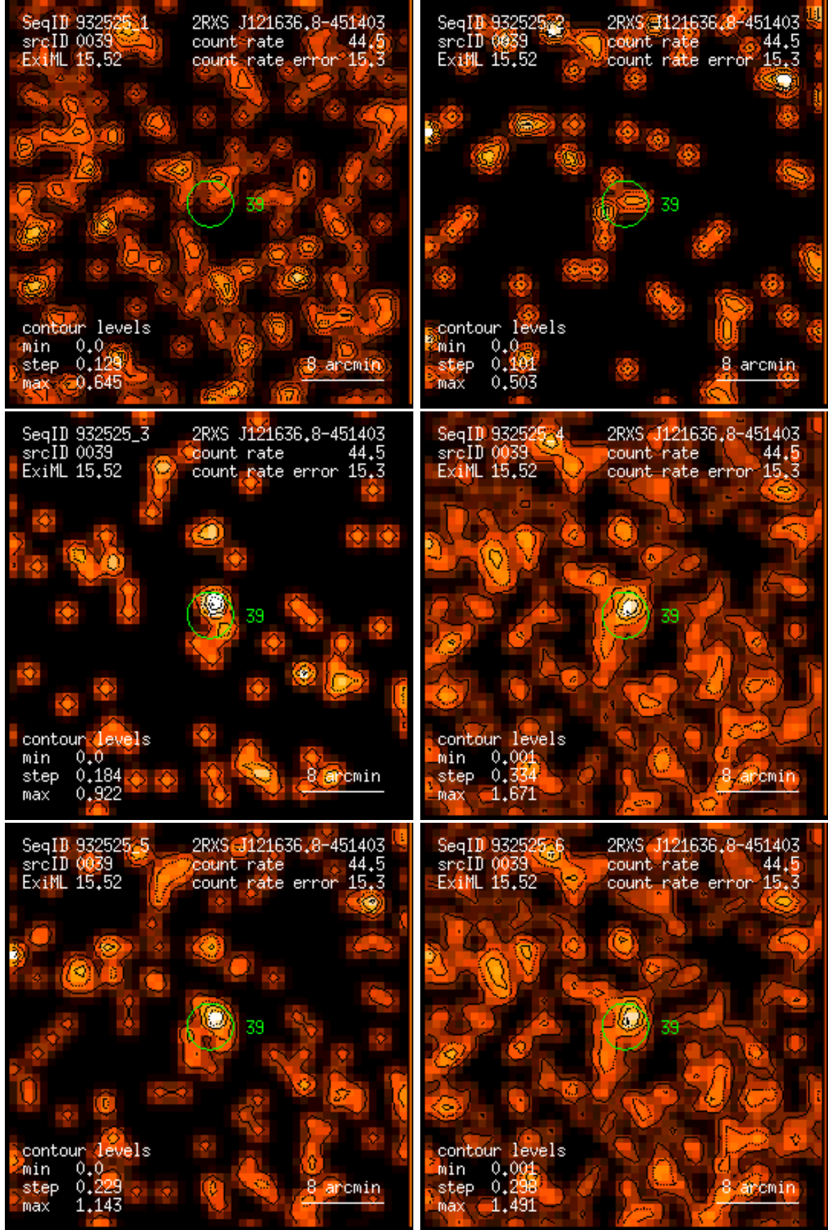
Figure 39: RASS 932525: detection 0039: band rate images, Gaussian filter: (1) PSPC channels 11 – 41, (2) 52 – 90, (3) 91 – 201, (4) 11 – 235, (5) 52 – 201, (6) 11 – 201. Broad band rates in counts/ks. Band rate contour levels in counts/ks/arcmin 2 .
