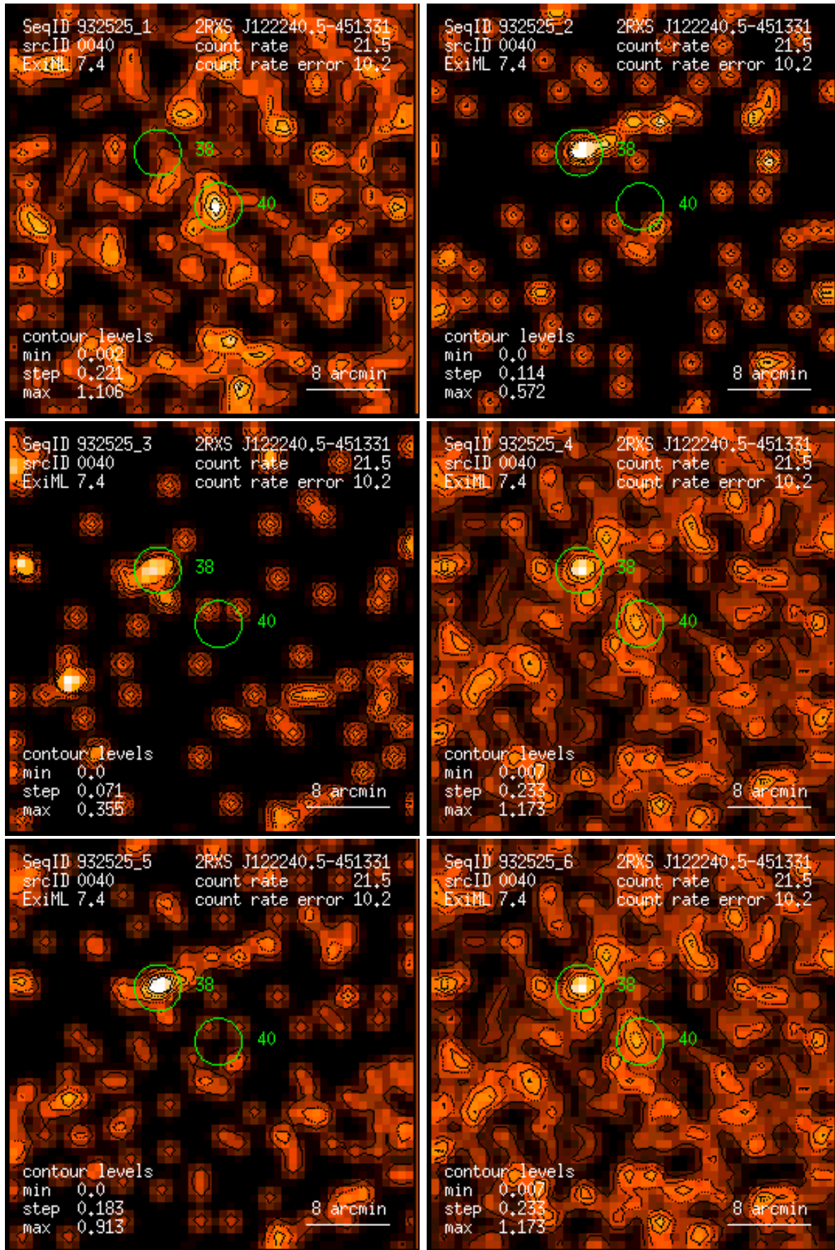
Figure 40: RASS 932525: detection 0040: band rate images, Gaussian filter: (1) PSPC channels 11 – 41, (2) 52 – 90, (3) 91 – 201, (4) 11 – 235, (5) 52 – 201, (6) 11 – 201. Broad band rates in counts/ks. Band rate contour levels in counts/ks/arcmin 2 .
