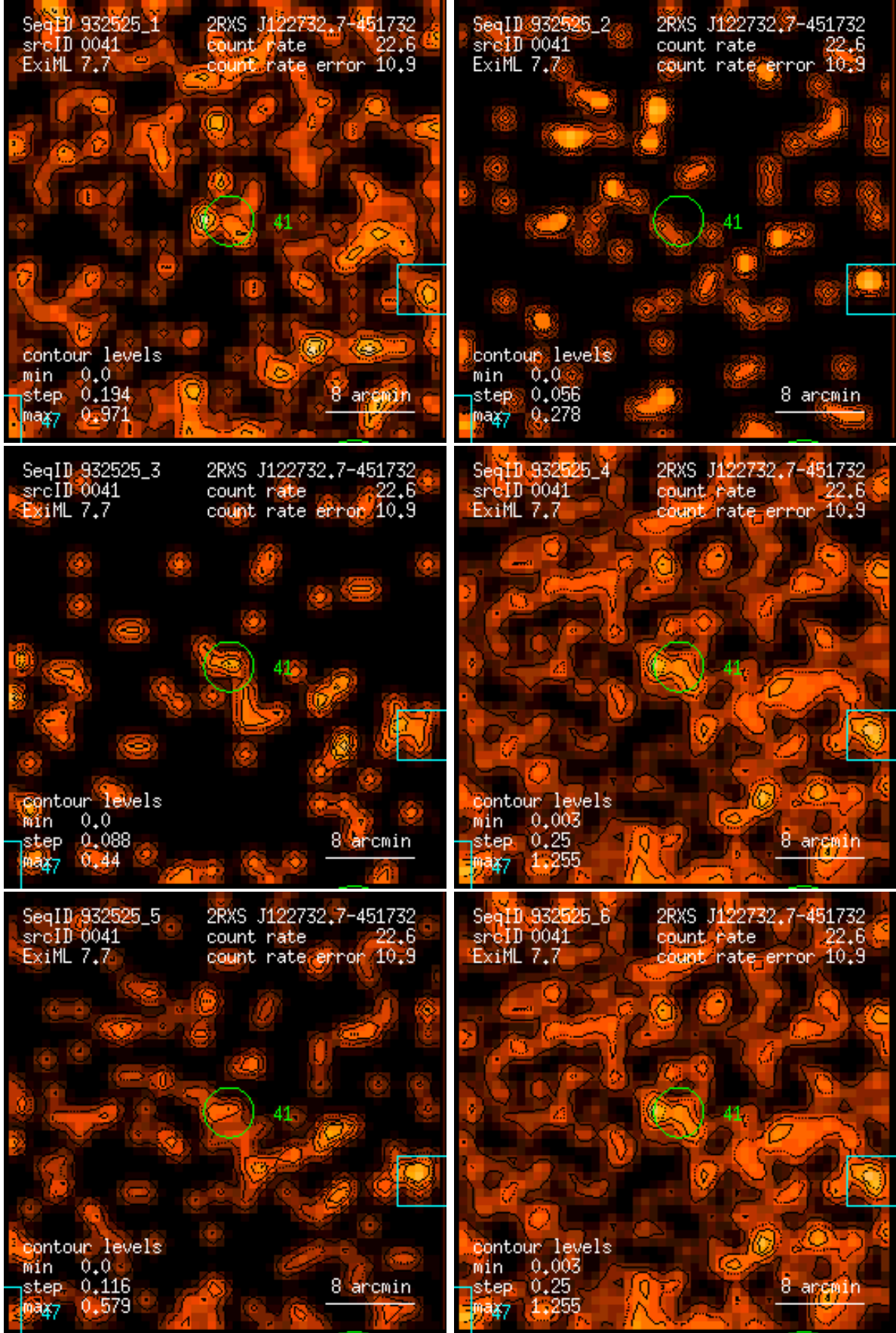
Figure 41: RASS 932525: detection 0041: band rate images, Gaussian filter: (1) PSPC channels 11 – 41, (2) 52 – 90, (3) 91 – 201, (4) 11 – 235, (5) 52 – 201, (6) 11 – 201. Broad band rates in counts/ks. Band rate contour levels in counts/ks/arcmin 2 .
