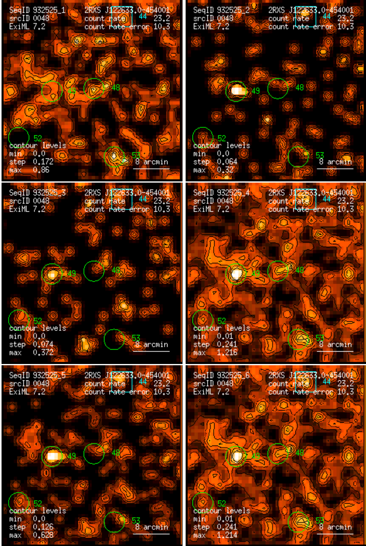
Figure 48: RASS 932525: detection 0048: band rate images, Gaussian filter: (1) PSPC channels 11 – 41, (2) 52 – 90, (3) 91 – 201, (4) 11 – 235, (5) 52 – 201, (6) 11 – 201. Broad band rates in counts/ks. Band rate contour levels in counts/ks/arcmin 2 .
