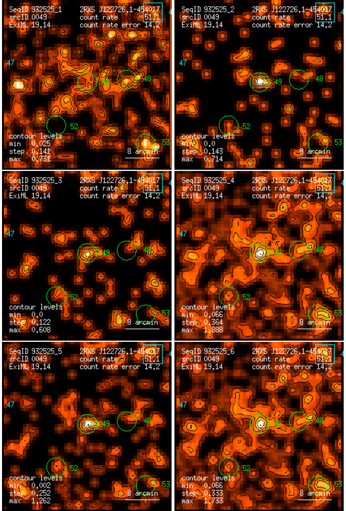
Figure 49: RASS 932525: detection 0049: band rate images, Gaussian filter: (1) PSPC channels 11 – 41, (2) 52 – 90, (3) 91 – 201, (4) 11 – 235, (5) 52 – 201, (6) 11 – 201. Broad band rates in counts/ks. Band rate contour levels in counts/ks/arcmin 2 .
