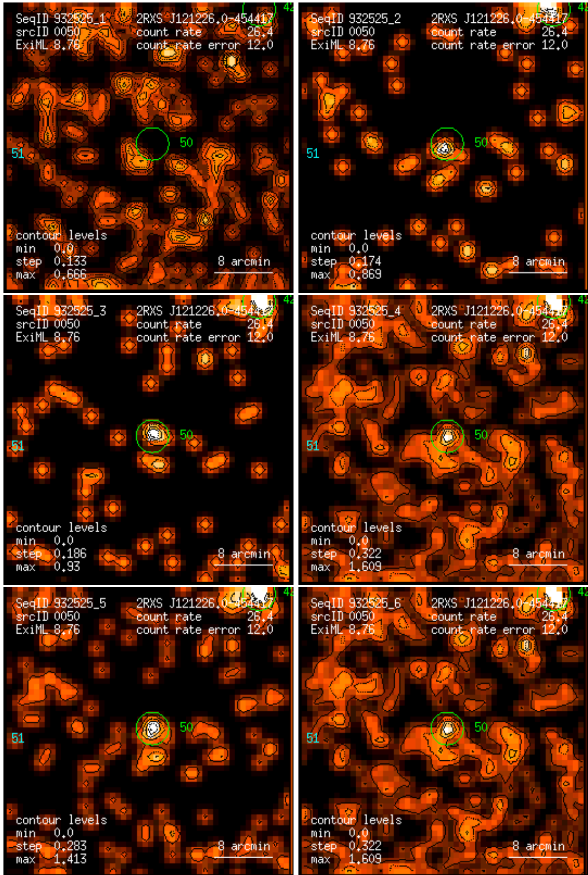
Figure 50: RASS 932525: detection 0050: band rate images, Gaussian filter: (1) PSPC channels 11 – 41, (2) 52 – 90, (3) 91 – 201, (4) 11 – 235, (5) 52 – 201, (6) 11 – 201. Broad band rates in counts/ks. Band rate contour levels in counts/ks/arcmin 2 .
