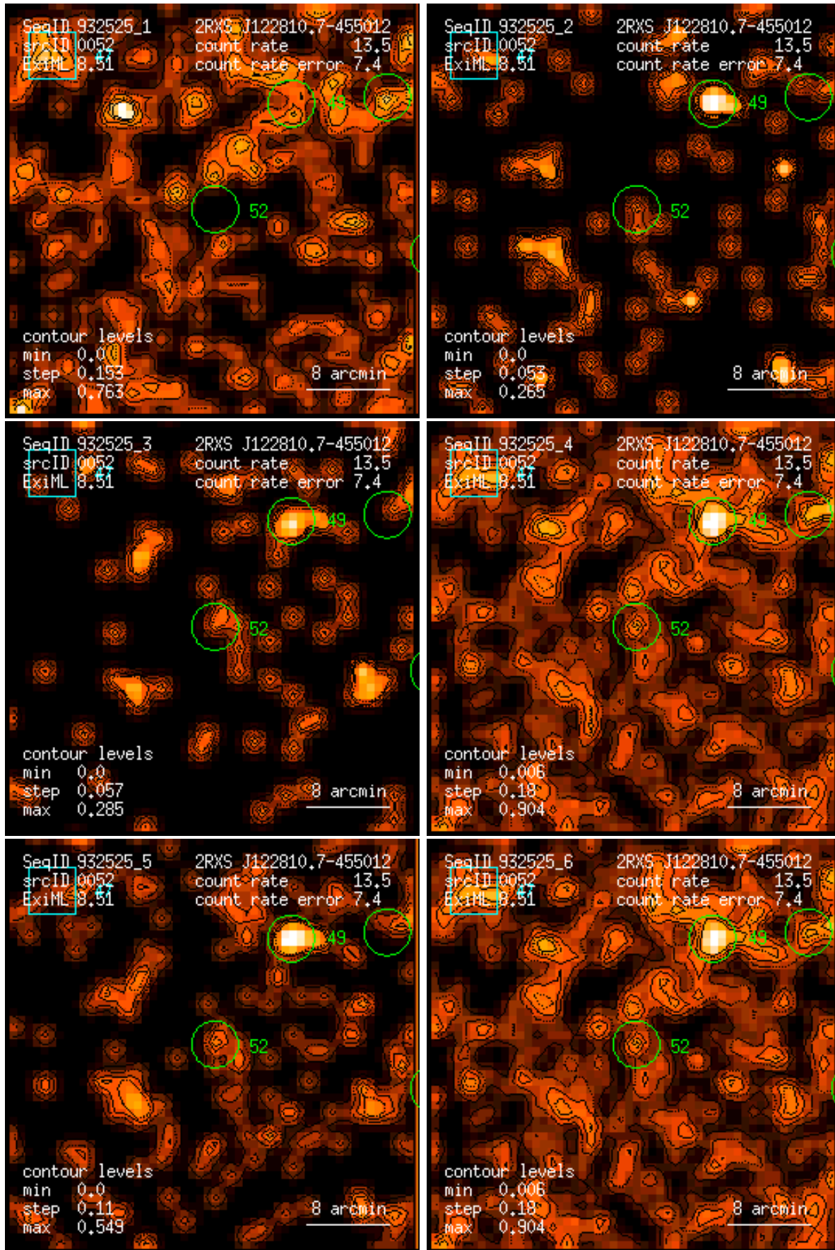
Figure 52: RASS 932525: detection 0052: band rate images, Gaussian filter: (1) PSPC channels 11 – 41, (2) 52 – 90, (3) 91 – 201, (4) 11 – 235, (5) 52 – 201, (6) 11 – 201. Broad band rates in counts/ks. Band rate contour levels in counts/ks/arcmin 2 .
