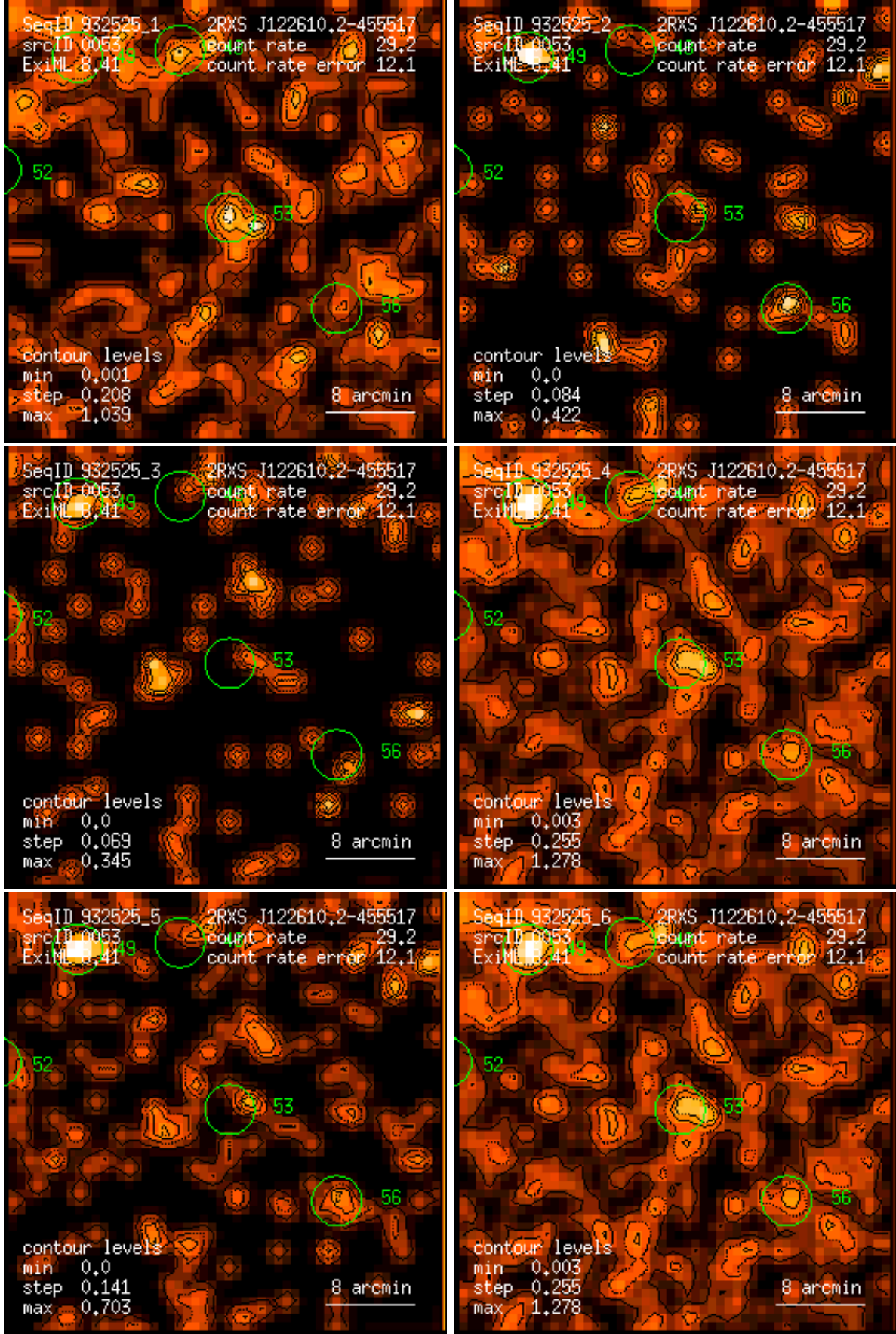
Figure 53: RASS 932525: detection 0053: band rate images, Gaussian filter: (1) PSPC channels 11 – 41, (2) 52 – 90, (3) 91 – 201, (4) 11 – 235, (5) 52 – 201, (6) 11 – 201. Broad band rates in counts/ks. Band rate contour levels in counts/ks/arcmin 2 .
