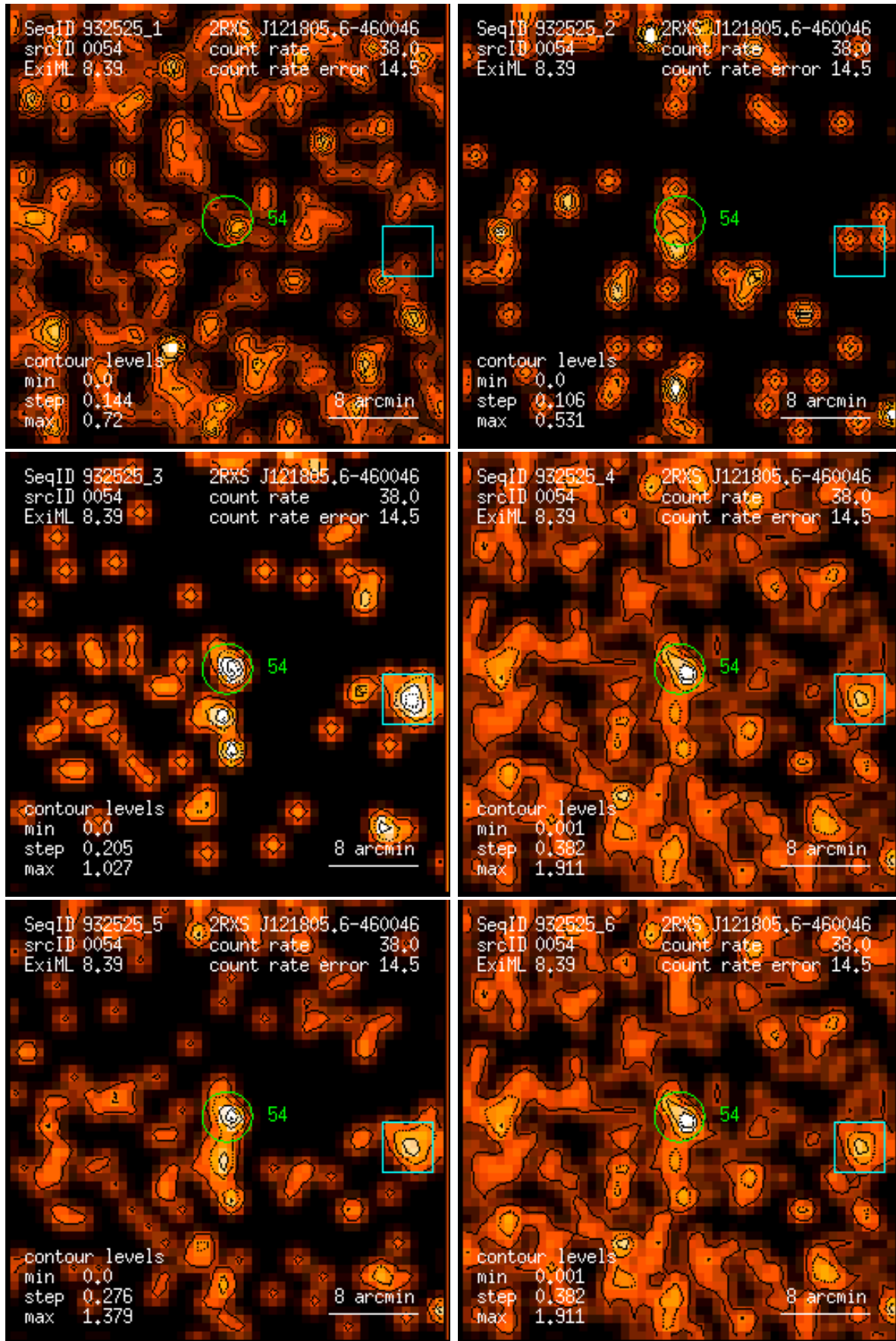
Figure 54: RASS 932525: detection 0054: band rate images, Gaussian filter: (1) PSPC channels 11 – 41, (2) 52 – 90, (3) 91 – 201, (4) 11 – 235, (5) 52 – 201, (6) 11 – 201. Broad band rates in counts/ks. Band rate contour levels in counts/ks/arcmin 2 .
