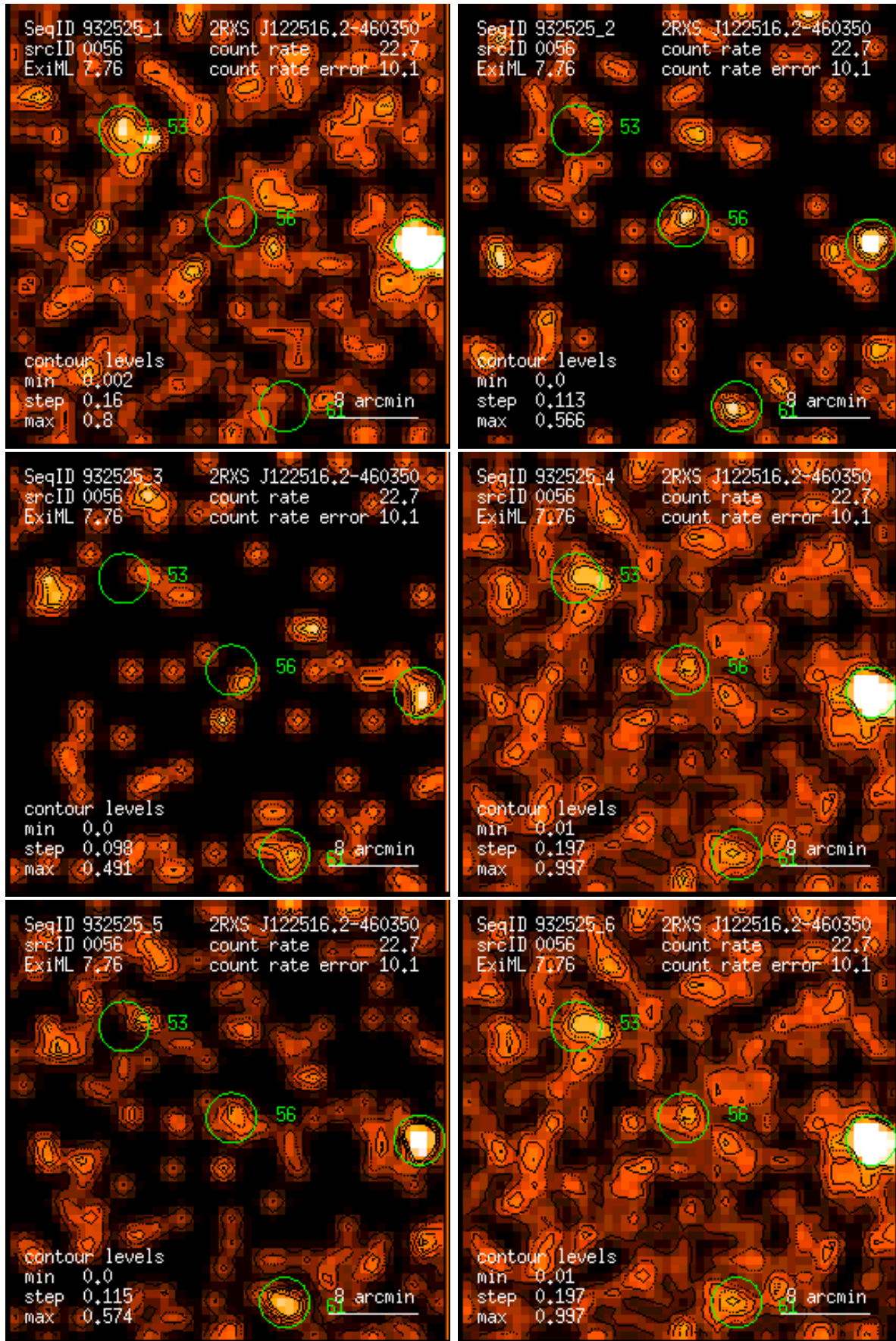
Figure 56: RASS 932525: detection 0056: band rate images, Gaussian filter: (1) PSPC channels 11 – 41, (2) 52 – 90, (3) 91 – 201, (4) 11 – 235, (5) 52 – 201, (6) 11 – 201. Broad band rates in counts/ks. Band rate contour levels in counts/ks/arcmin 2 .
