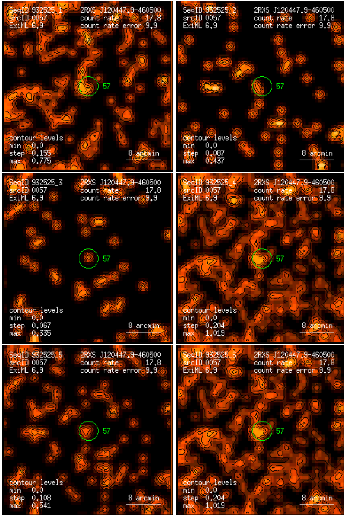
Figure 57: RASS 932525: detection 0057: band rate images, Gaussian filter: (1) PSPC channels 11 – 41, (2) 52 – 90, (3) 91 – 201, (4) 11 – 235, (5) 52 – 201, (6) 11 – 201. Broad band rates in counts/ks. Band rate contour levels in counts/ks/arcmin 2 .
