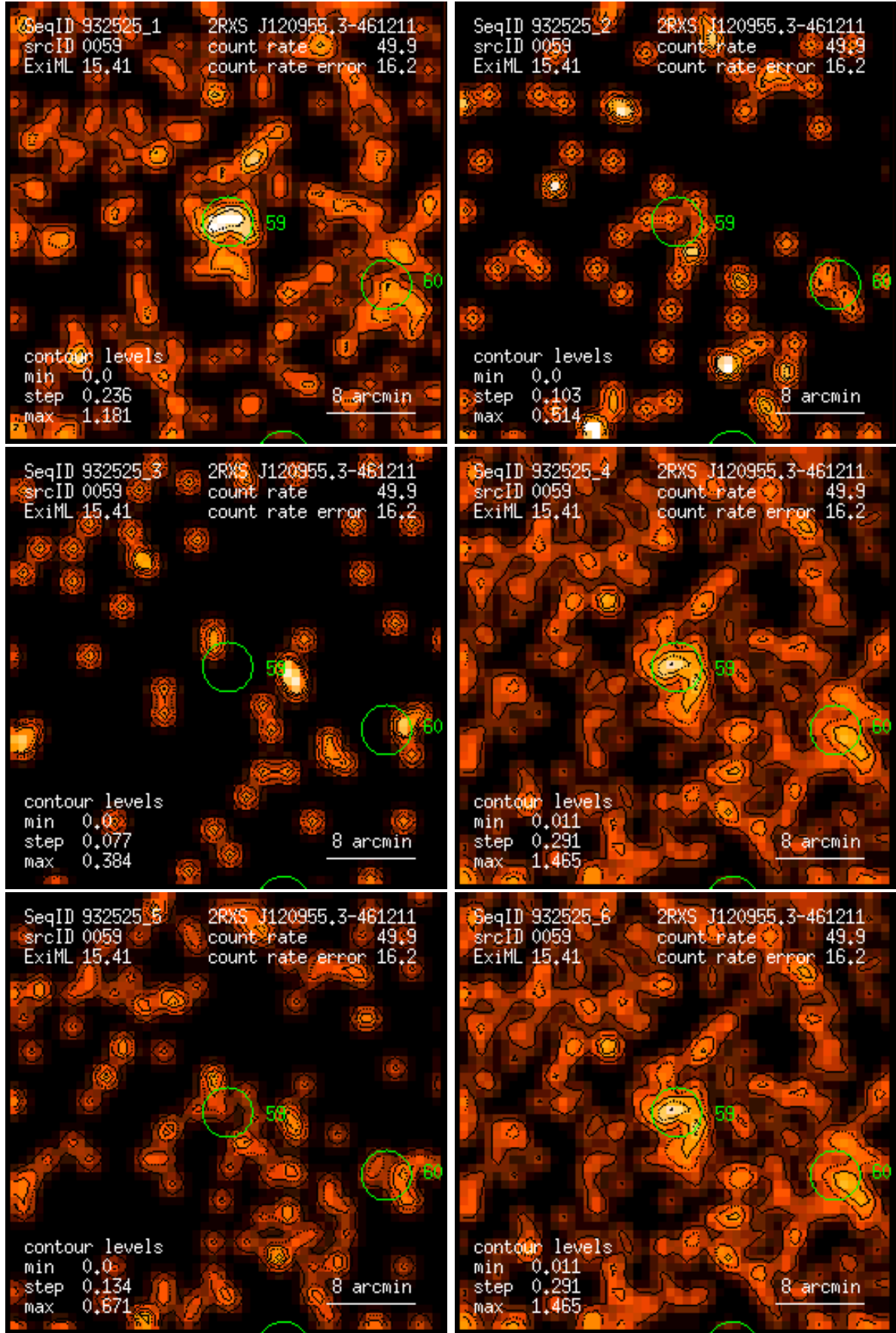
Figure 59: RASS 932525: detection 0059: band rate images, Gaussian filter: (1) PSPC channels 11 – 41, (2) 52 – 90, (3) 91 – 201, (4) 11 – 235, (5) 52 – 201, (6) 11 – 201. Broad band rates in counts/ks. Band rate contour levels in counts/ks/arcmin 2 .
